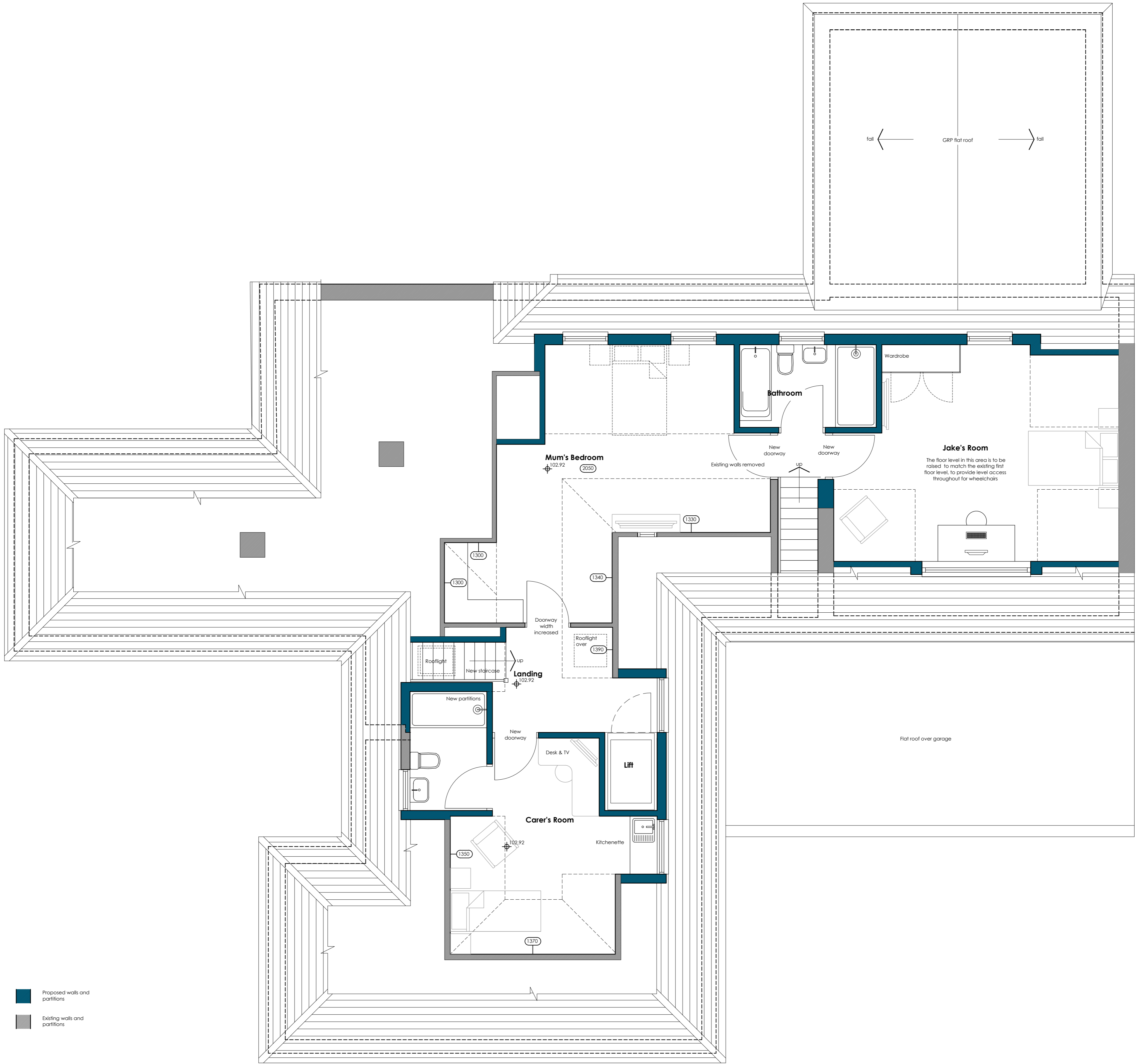
Proposed First Floor Plan, 1:50
