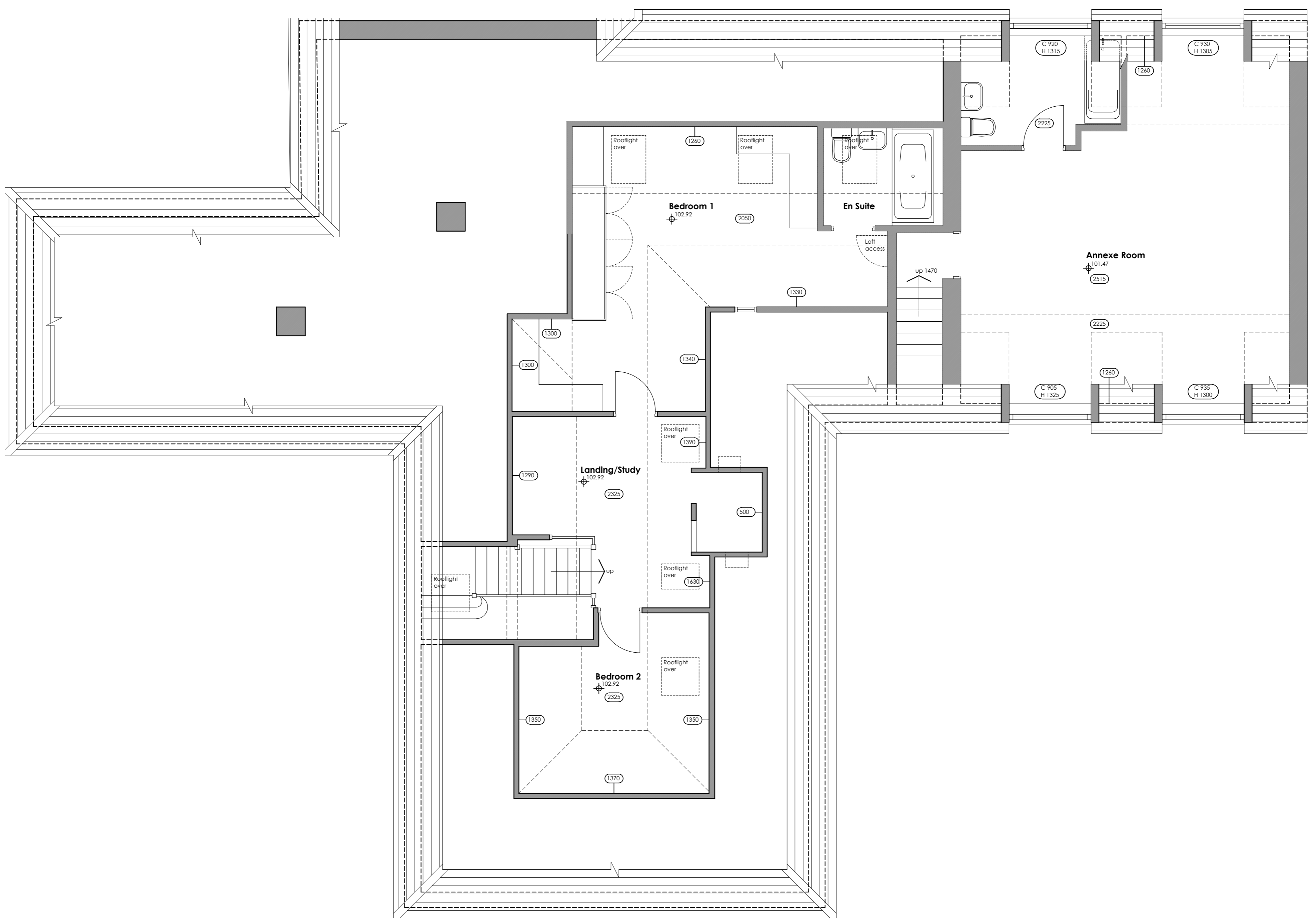
Existing First Floor Plan, 1:50
