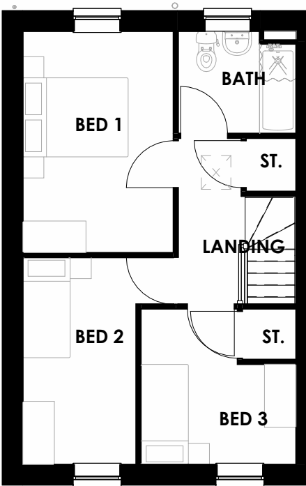
FIRST FLOOR PLANNING 1 : 100
