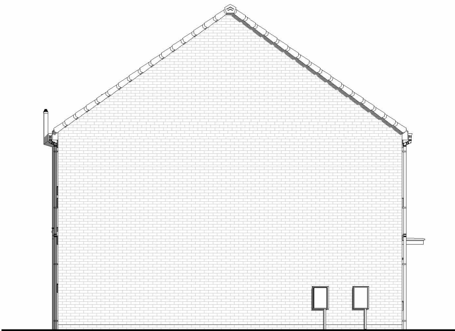
LEFT ELEVATION 1 : 100
