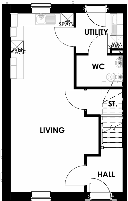
GROUND FLOOR PLANNING 1 : 100
