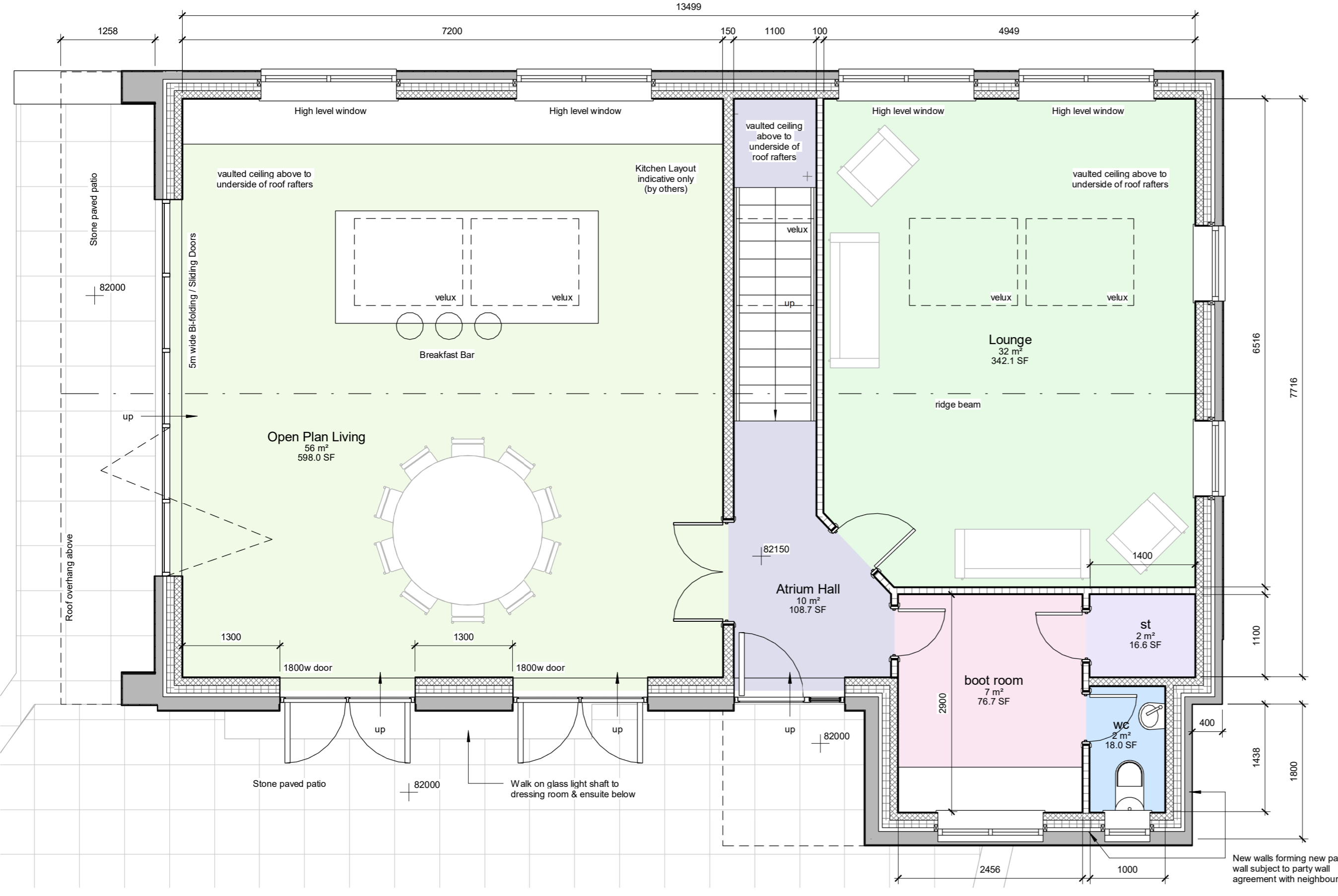
Proposed GF 1 : 50
