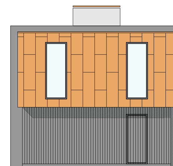
NORTH ELEVATION 1:100
