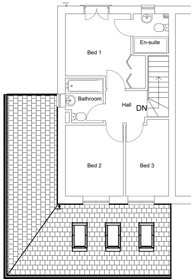
1 03b FF Proposed 1 : 100
