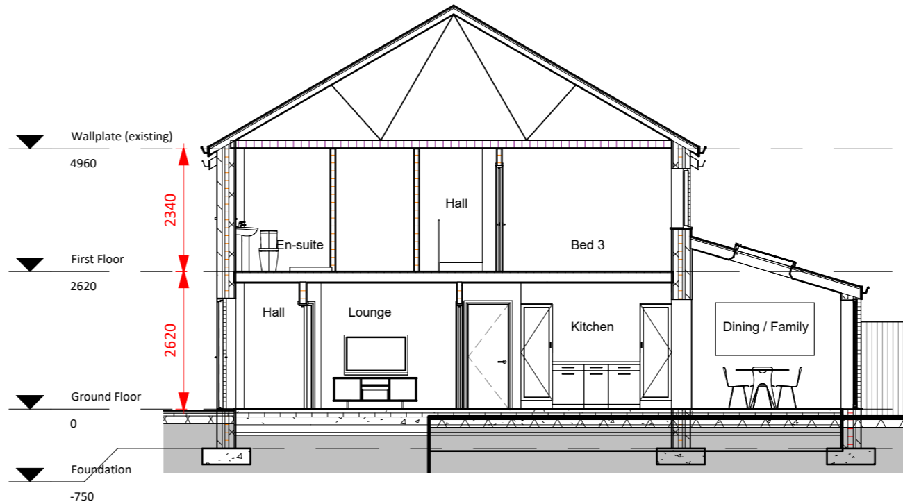
2 Proposed Section 1 : 100
