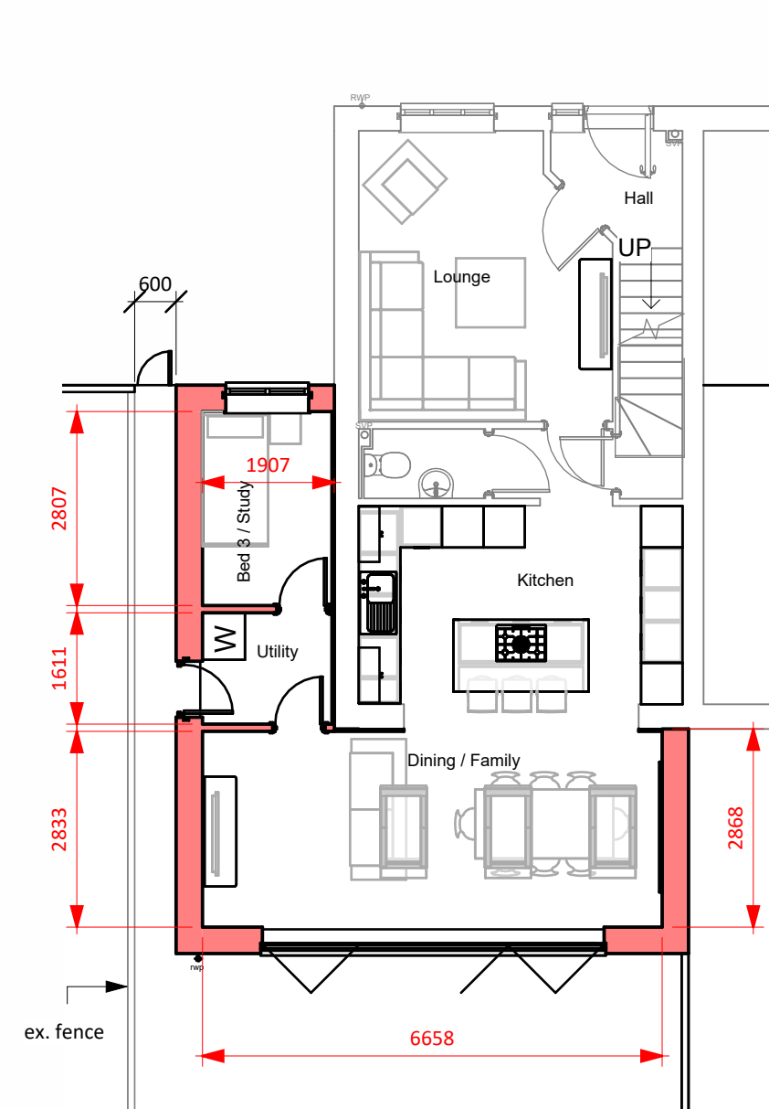
1 02b GF Proposed 1 : 100
