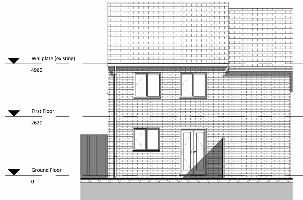
2 10 South Existing 1 : 100
