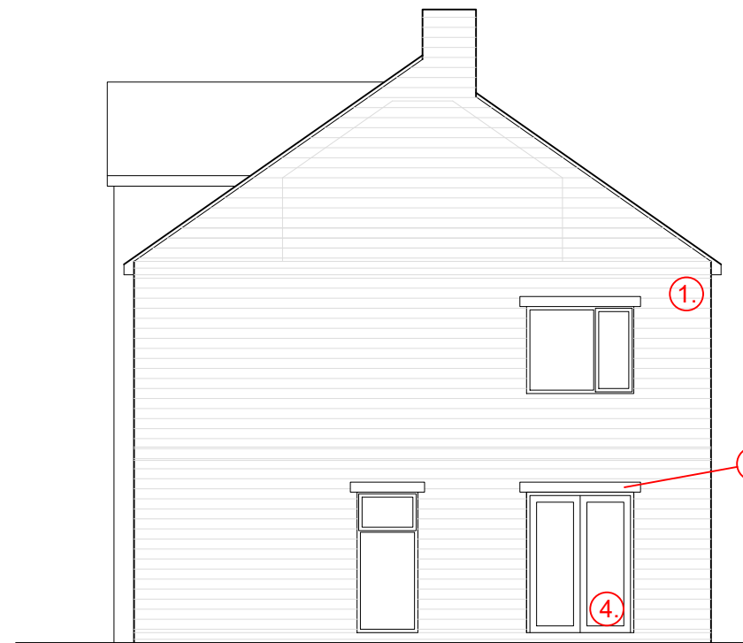
Elevation B Side (1.100 @ A3)
