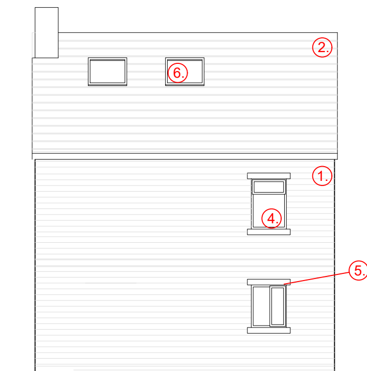
Elevation C Rear (1.100 @ A3)
