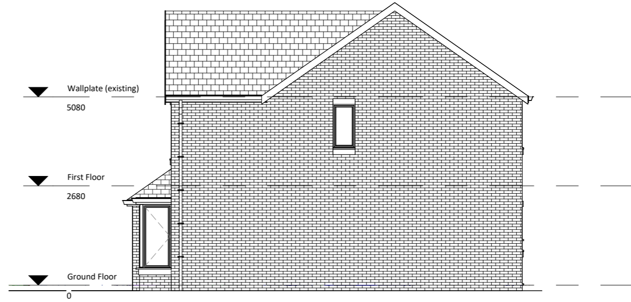
2 10 Existing East Elevation 1 : 100
