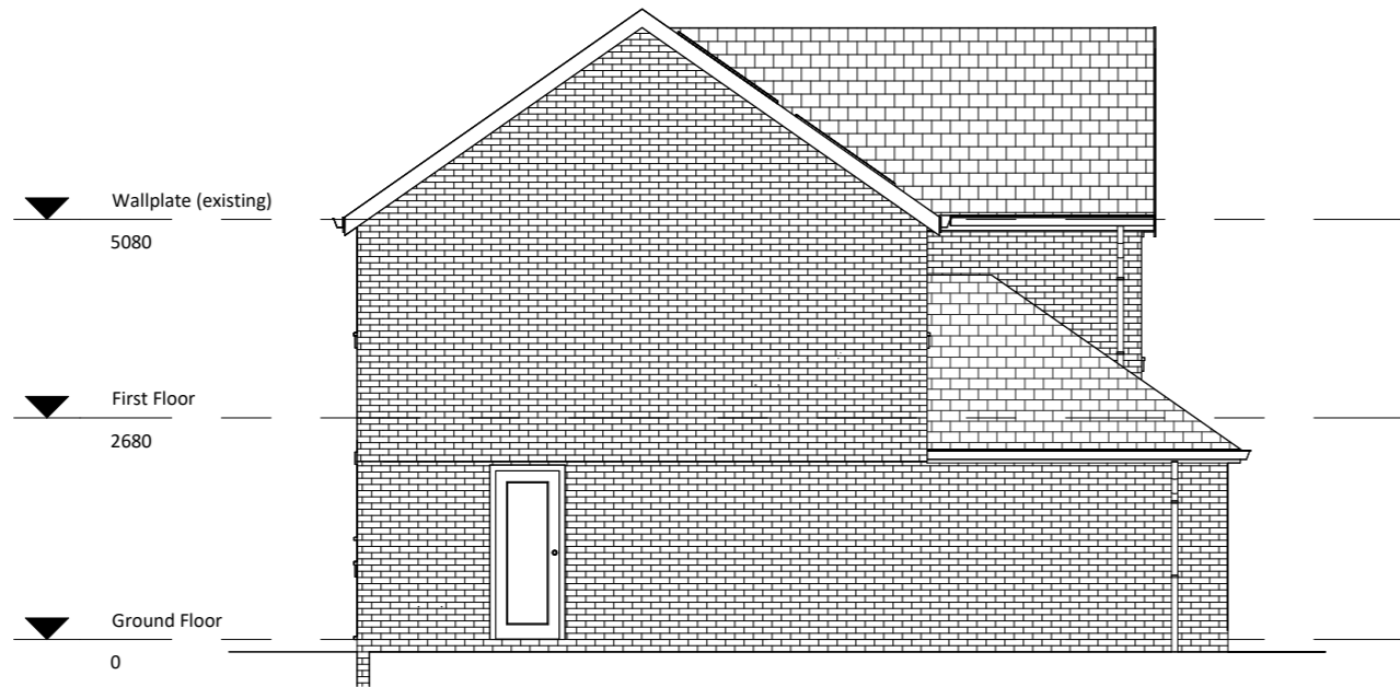
3 10 Existing West Elevation 1 : 100
