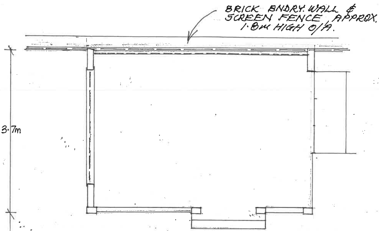
FLOOR PLAN
