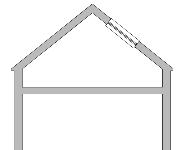
Section 1:100
