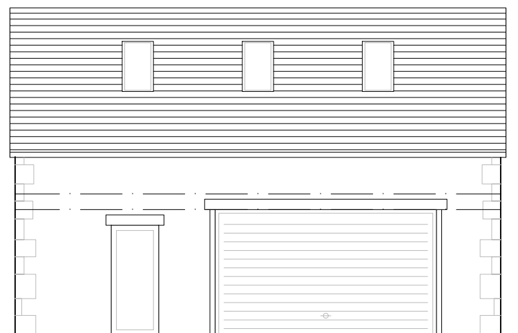
Front Elevation 1:100
