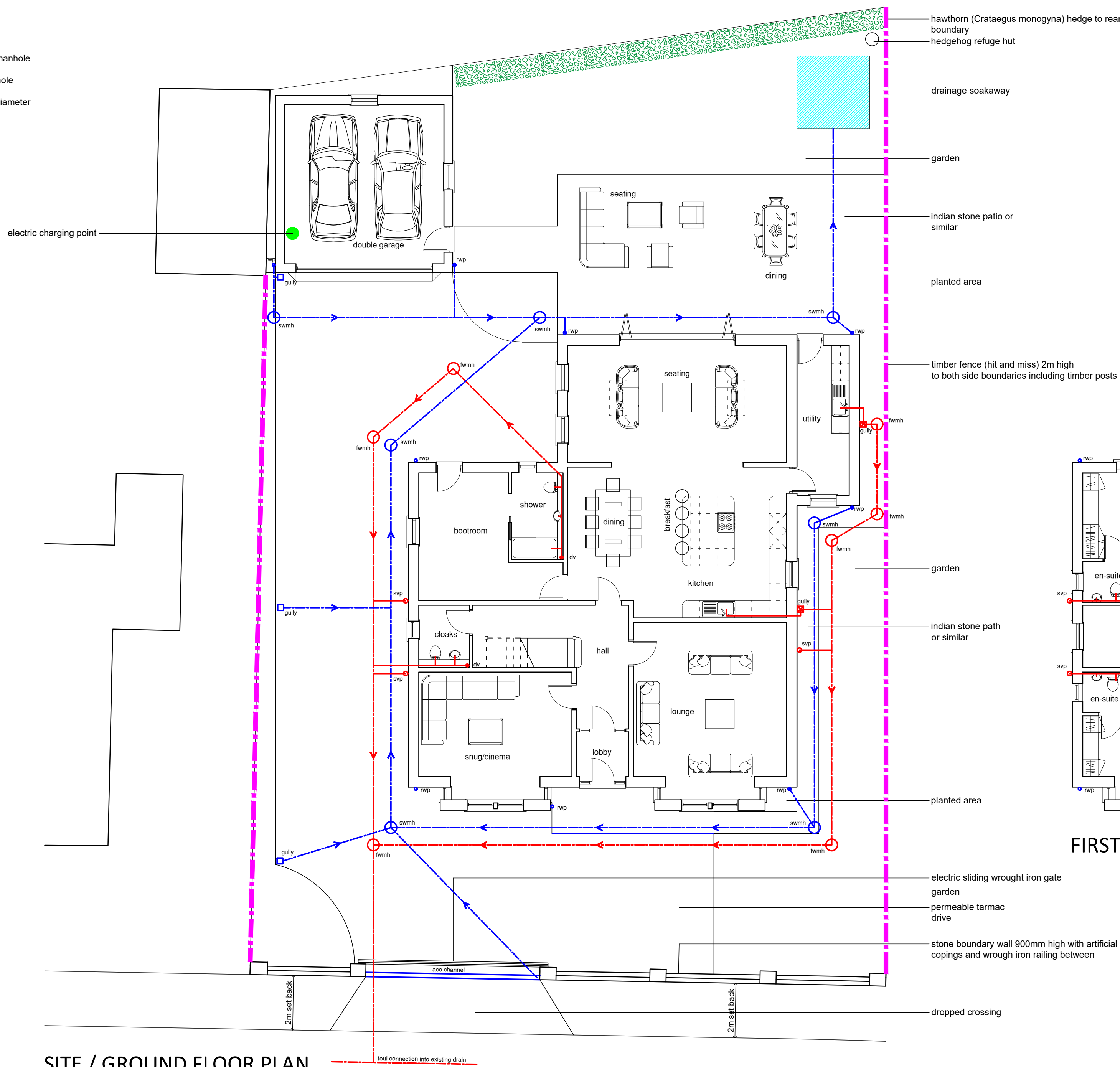
SITE / GROUND FLOOR PLAN
