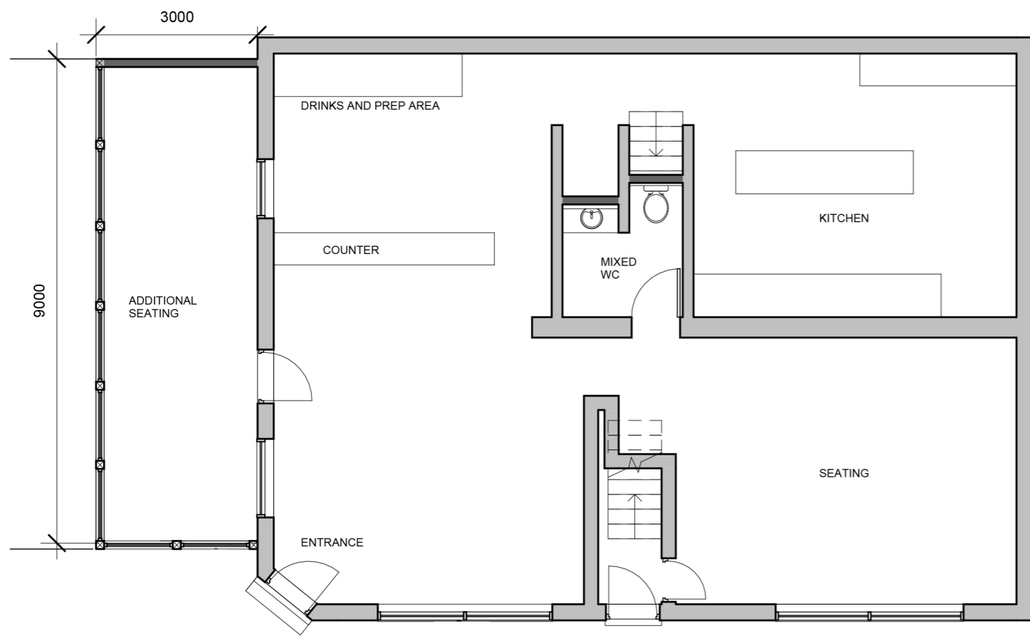
Ground Floor 1 : 100
