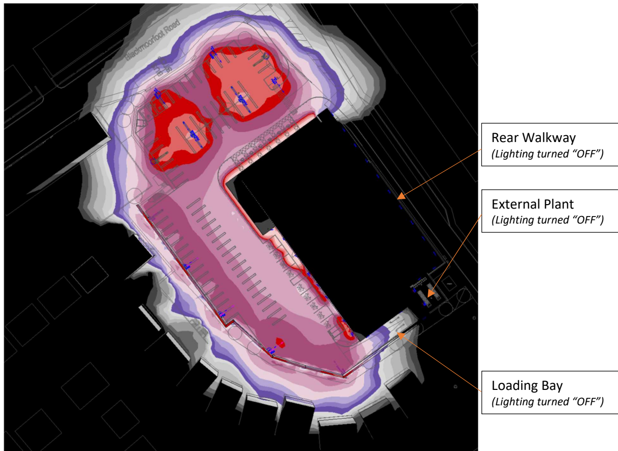
Fig 2. Building mounted luminaries to Rear store, Plant & Delivery area – Switched OFF
