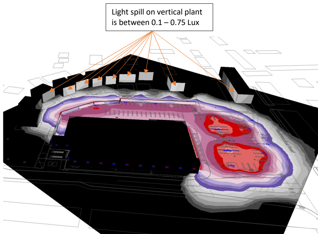
Fig 3b. Residential Area – False colour rendering - Residential Properties 1-11
