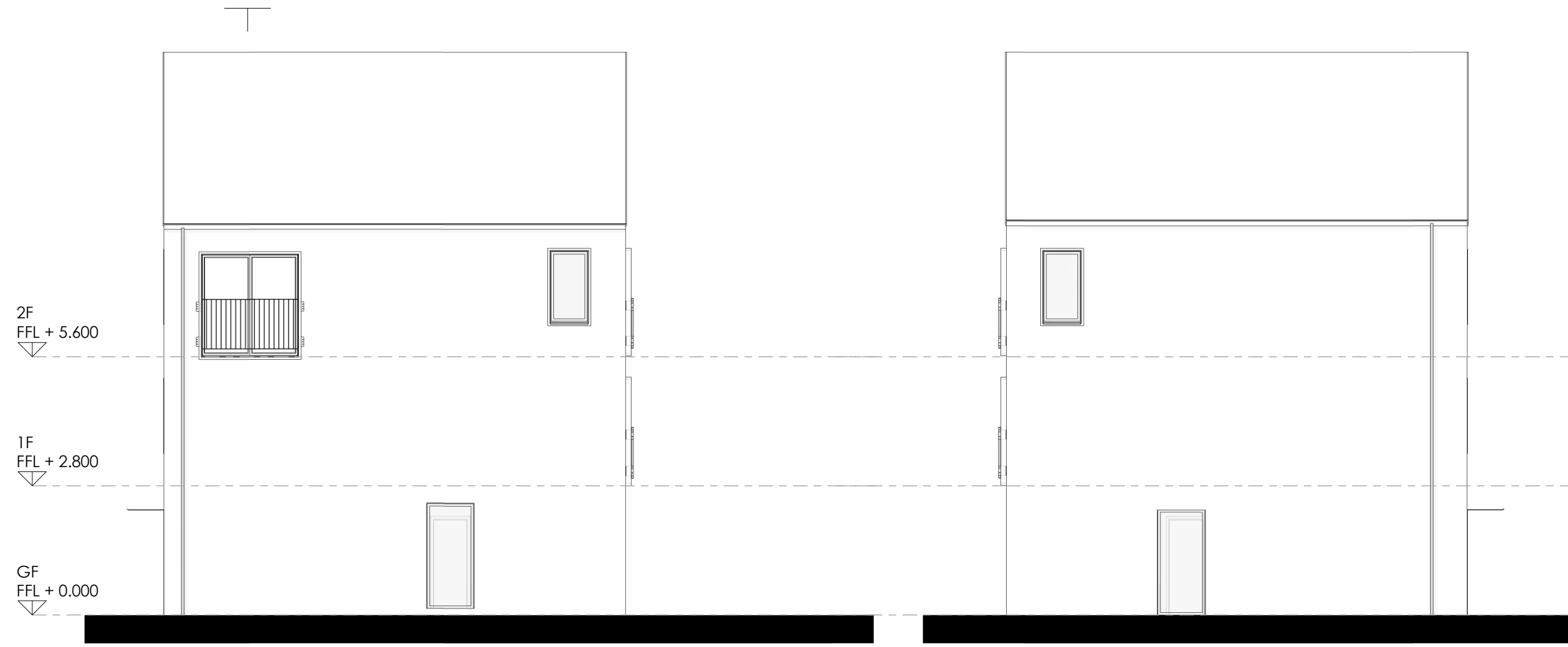
b - canalside north elevation
