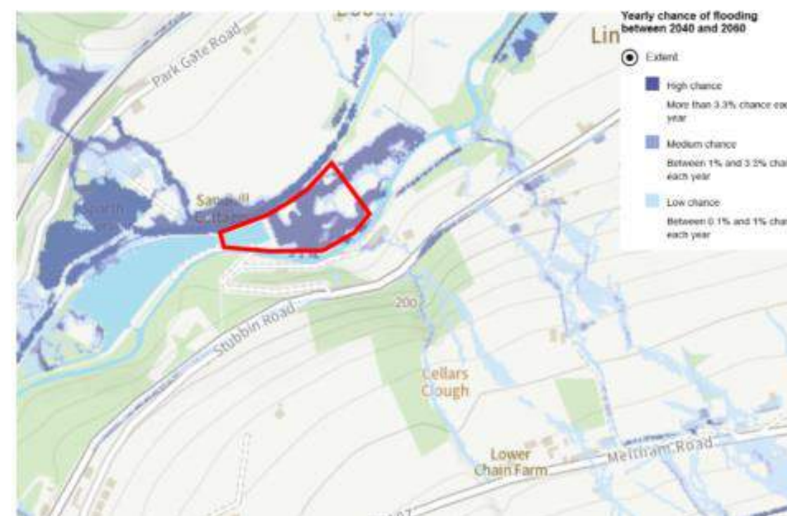
Figure 6: Environment Agency Risk of Flood From Surface Water – Climate Change Applied
