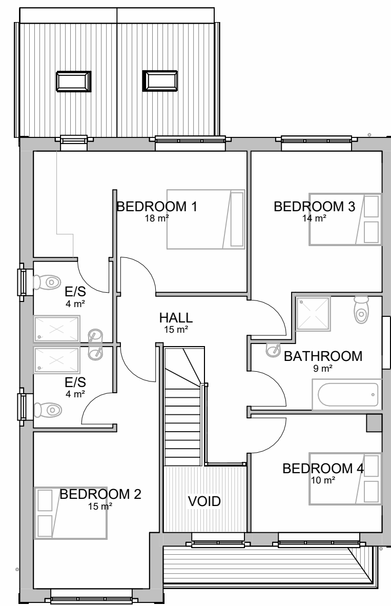
First Floor
