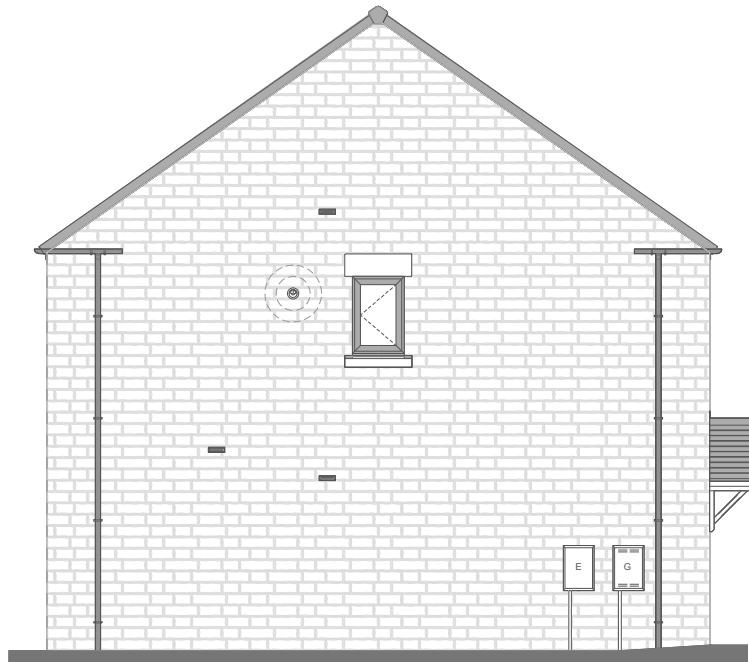
Left Elevation
