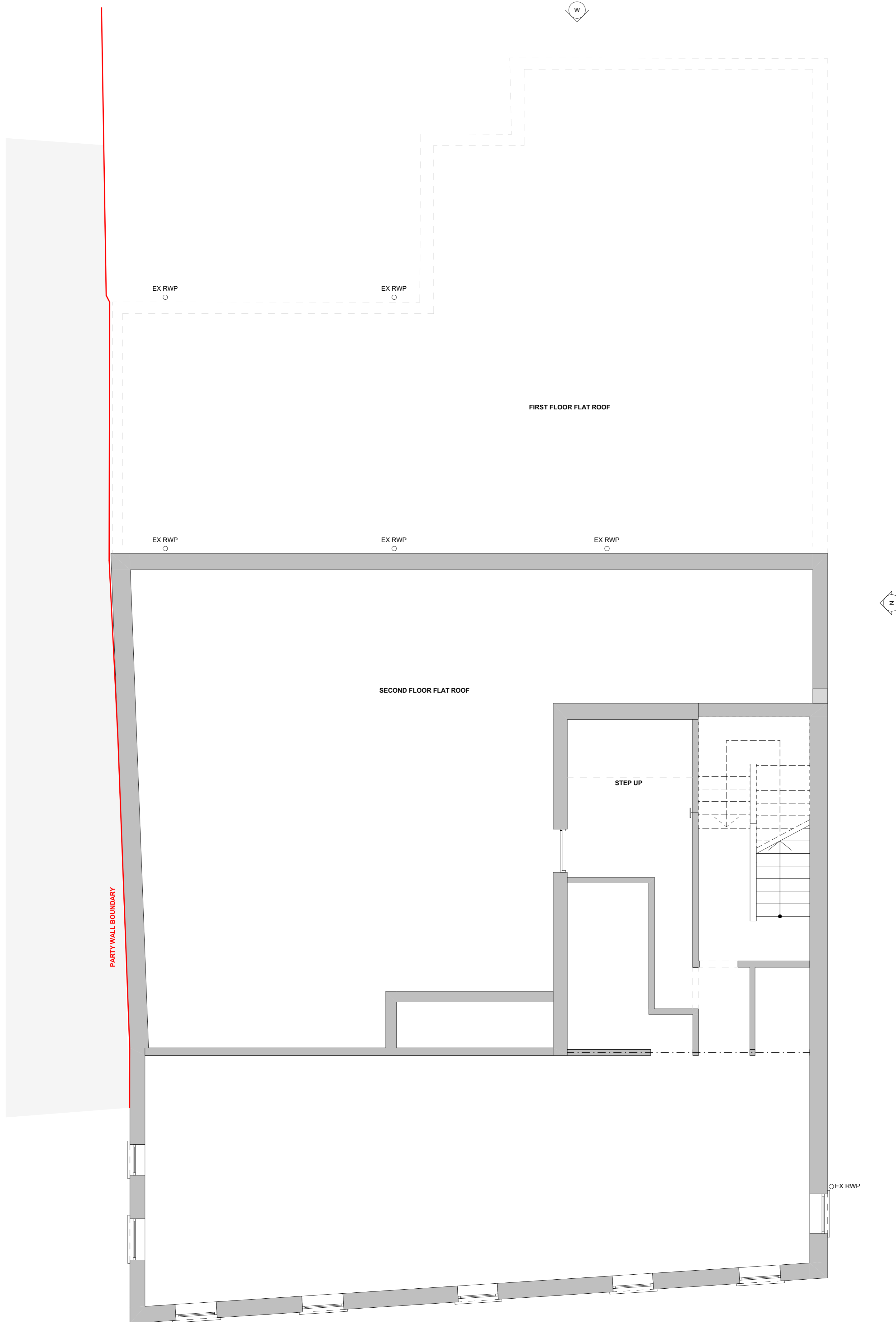
Existing Second Floor 1:50
