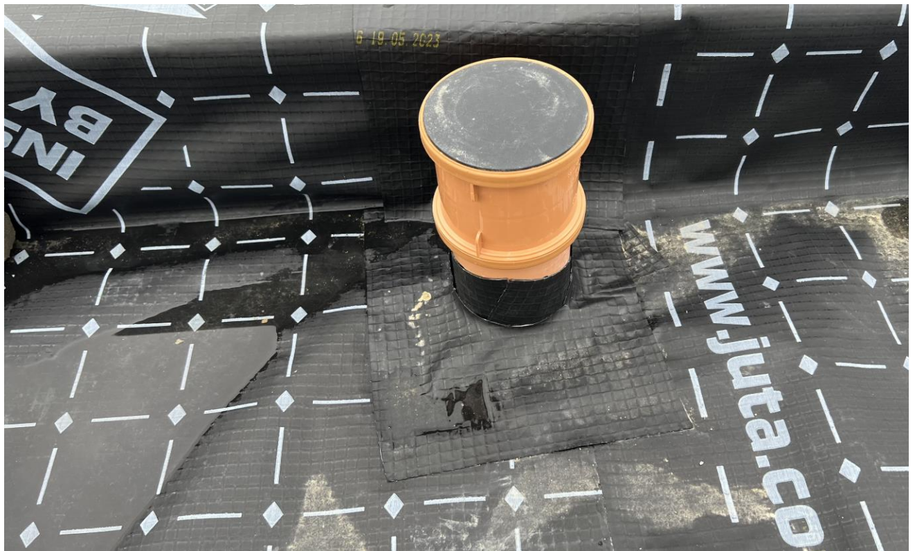
Plots 97 & 98 – Membrane layout with tophat and jointing
