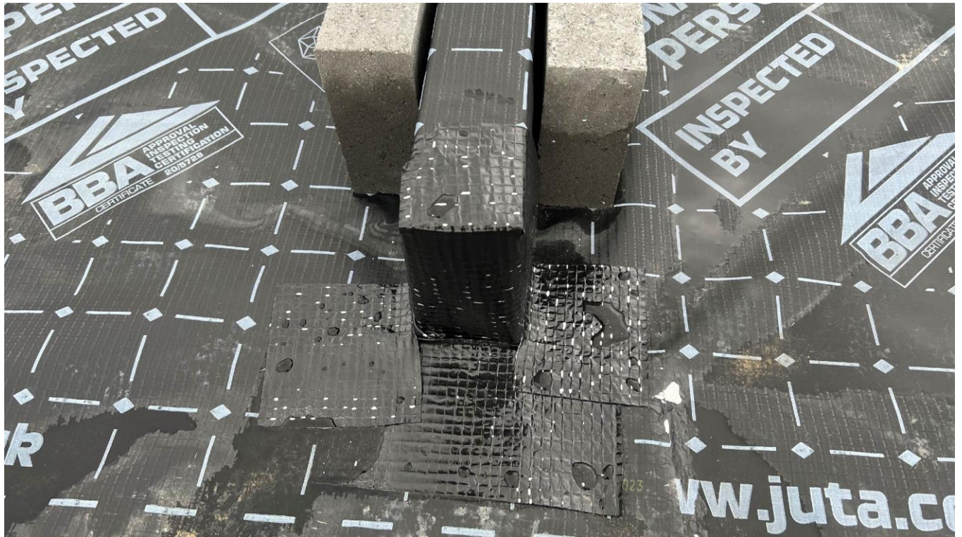
Plots 97 & 98 – Membrane layout with internal wall and jointing
