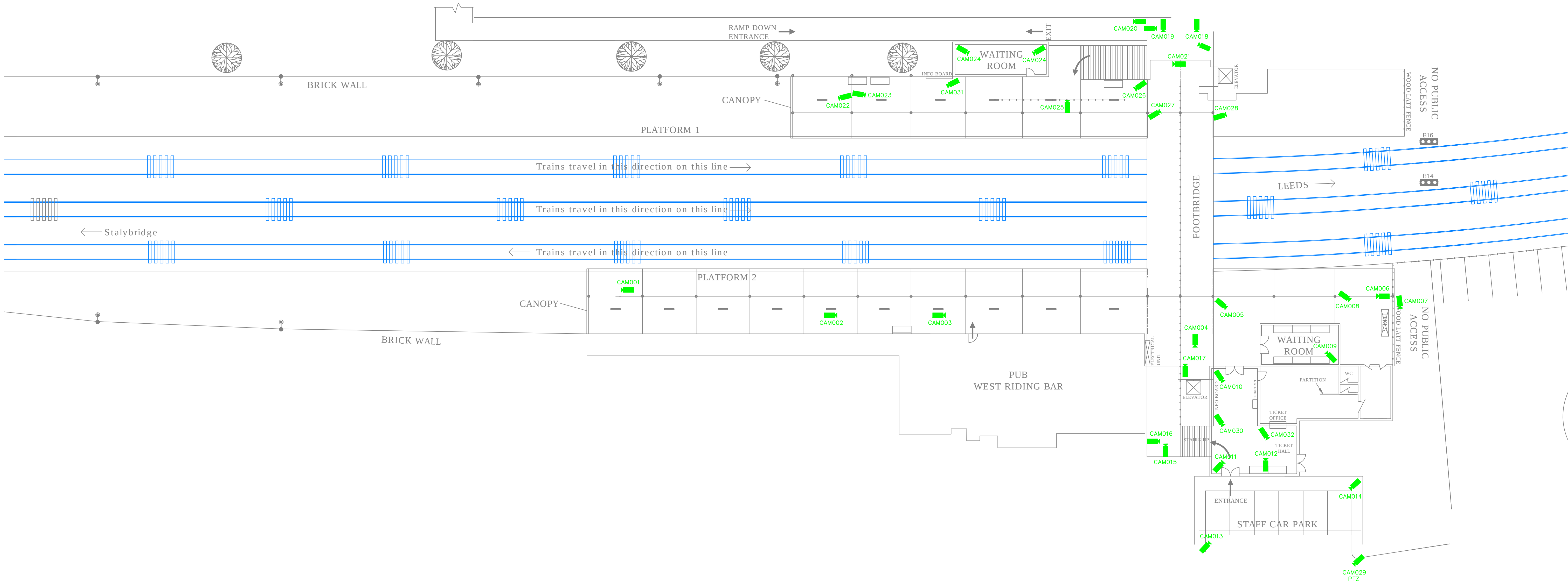
DEWSBURY STATION PLAN - PLATFORM LEVEL SCALE 1:200
