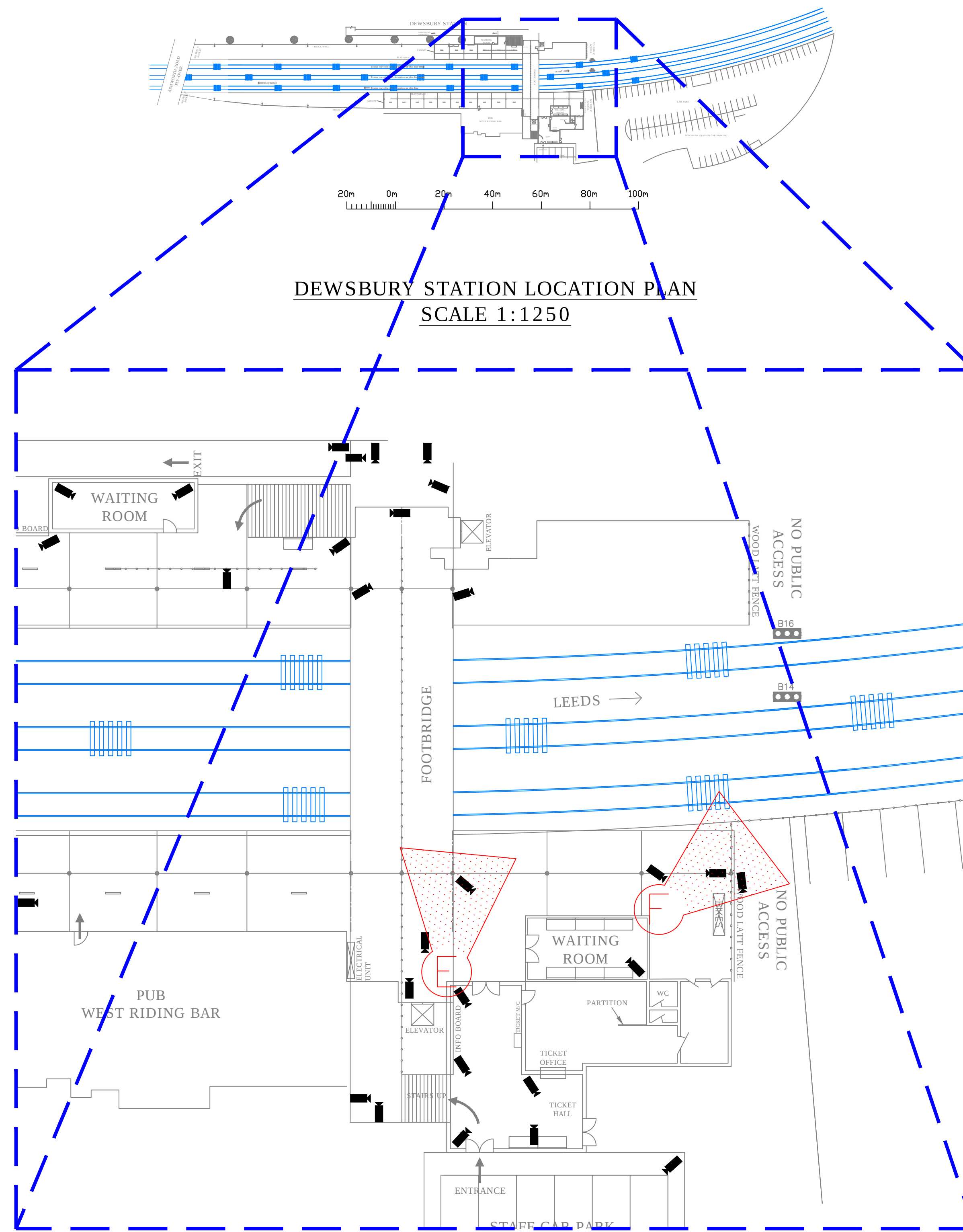
DEWSBURY STATION PLAN - PLATFORM LEVEL SCALE 1:200
