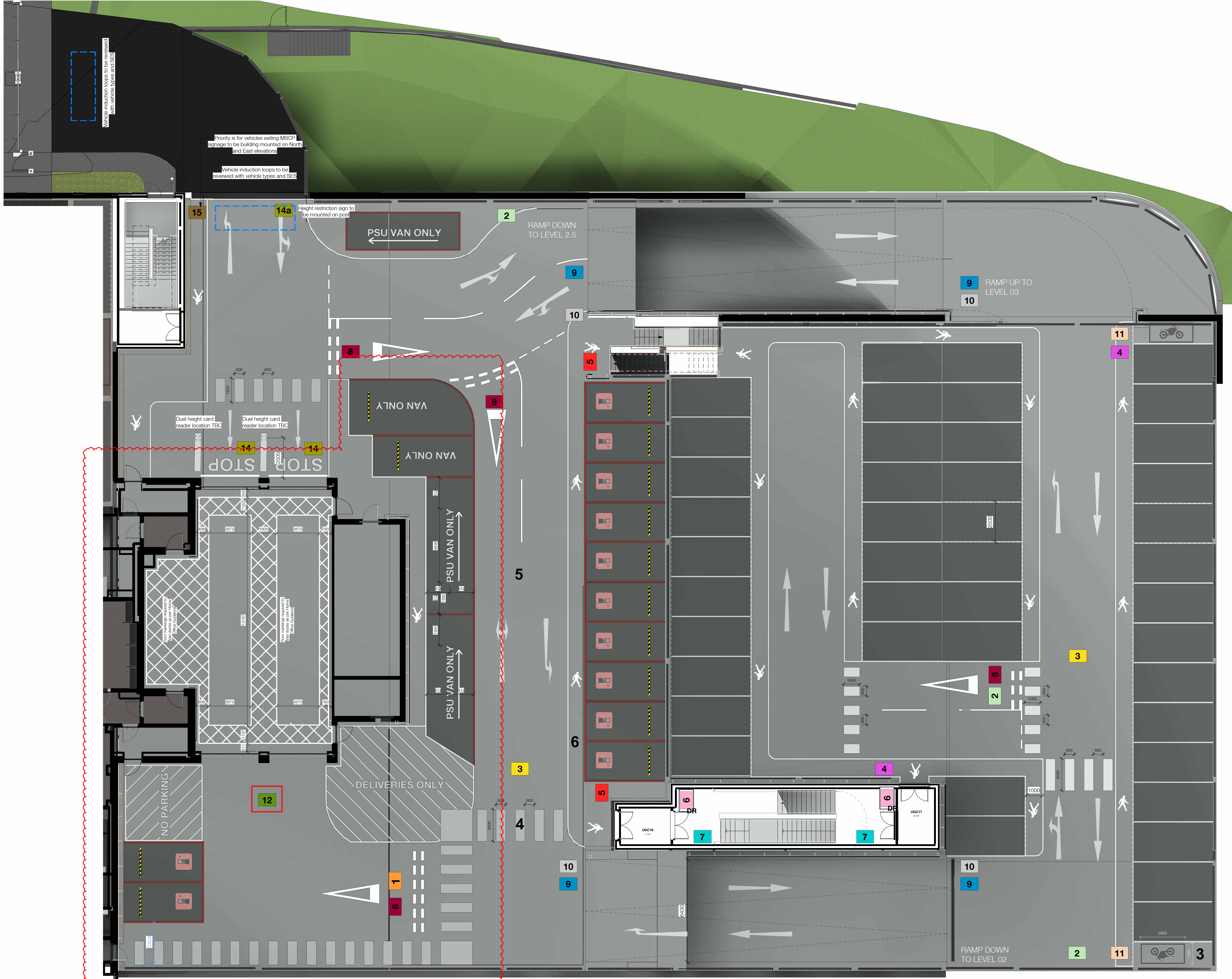
1 Road Markings Plan_CP Deck 2.5_3.0 1:100
