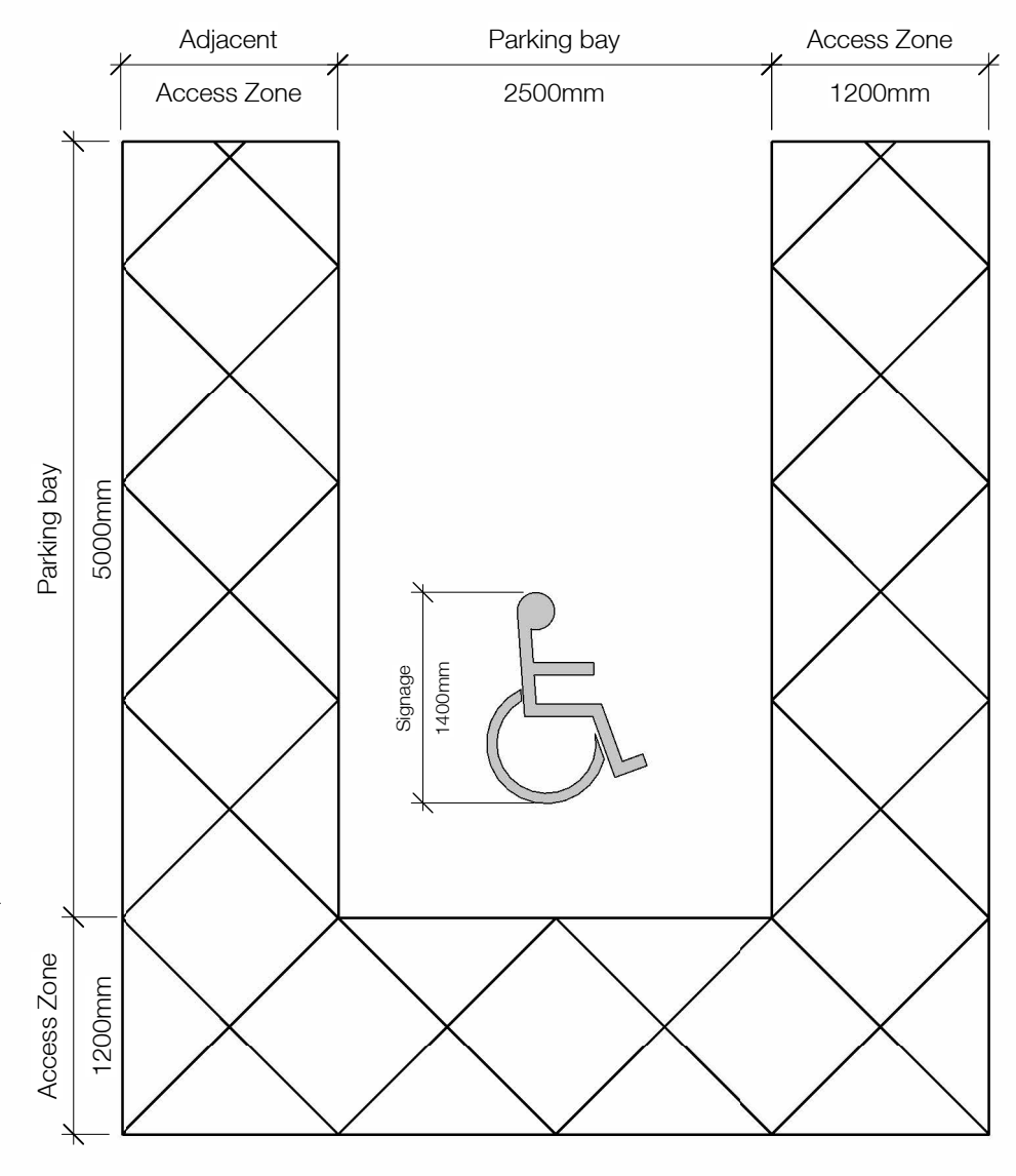
Road Marking sizes 1:25
