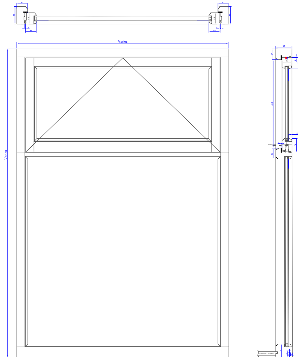
Rear elevation window
