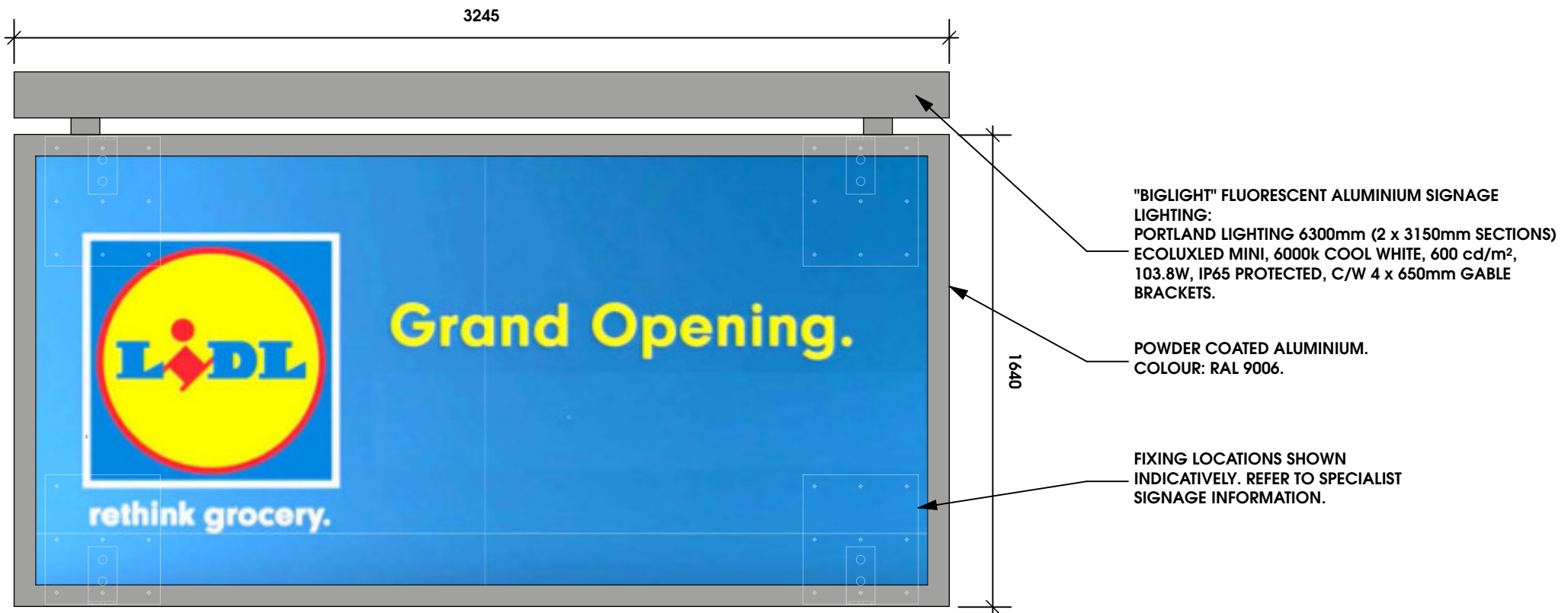
LIDL SMALL WALL MOUNTED BILLBOARD 1:20
