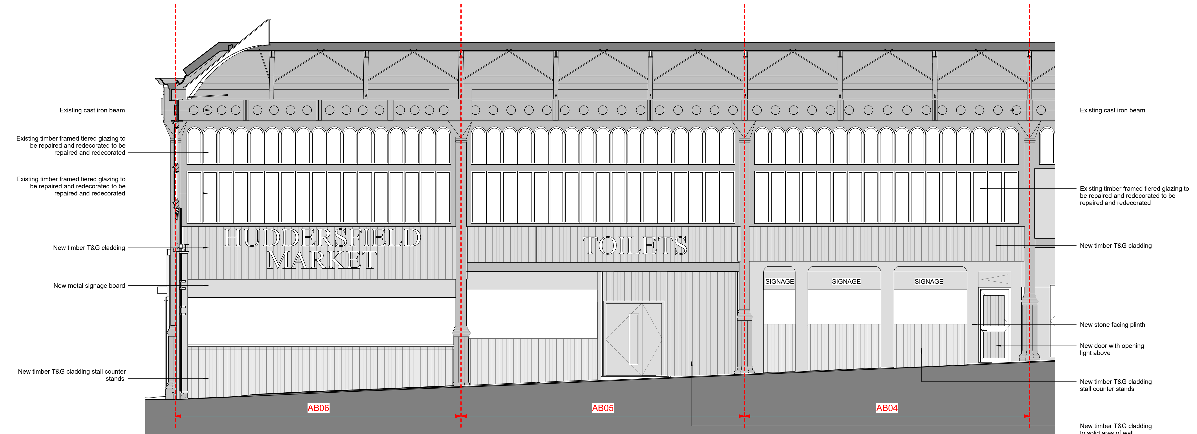
1 AB04-AB06 Internal Elevation 1 : 50
