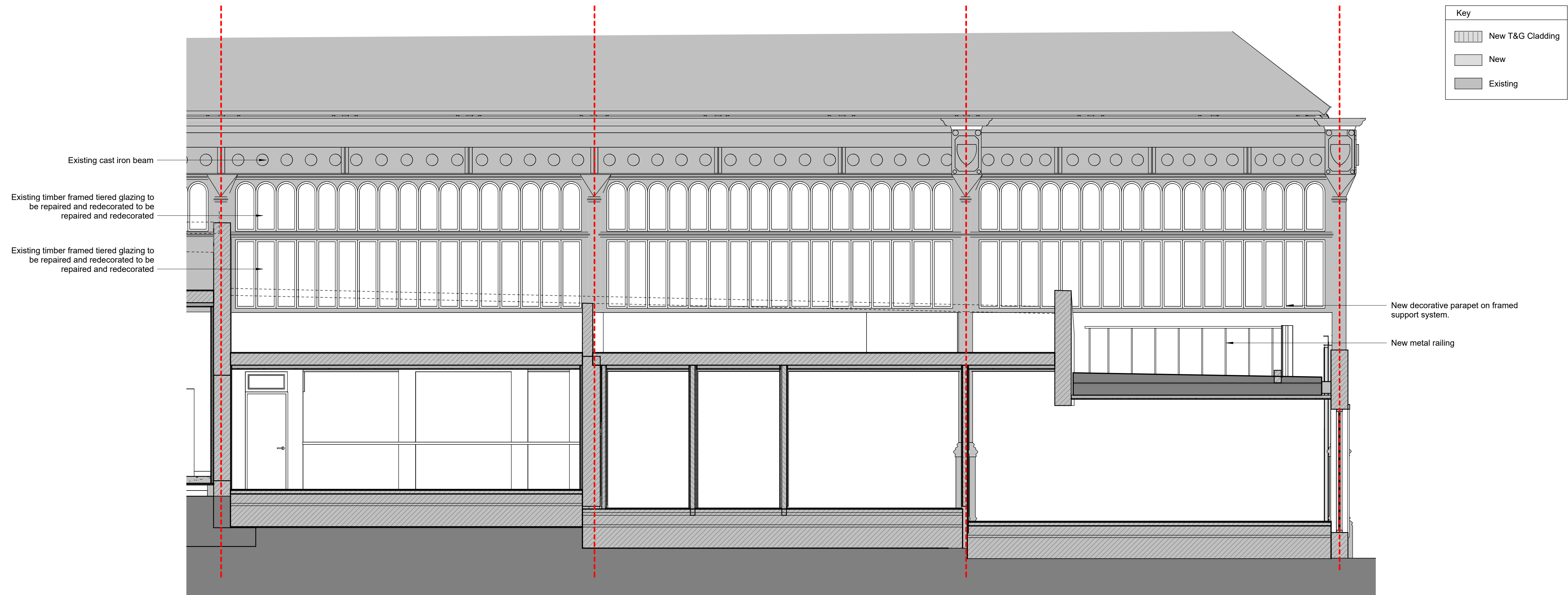
2 AB04 - AB06 External Elevation 1 : 50
