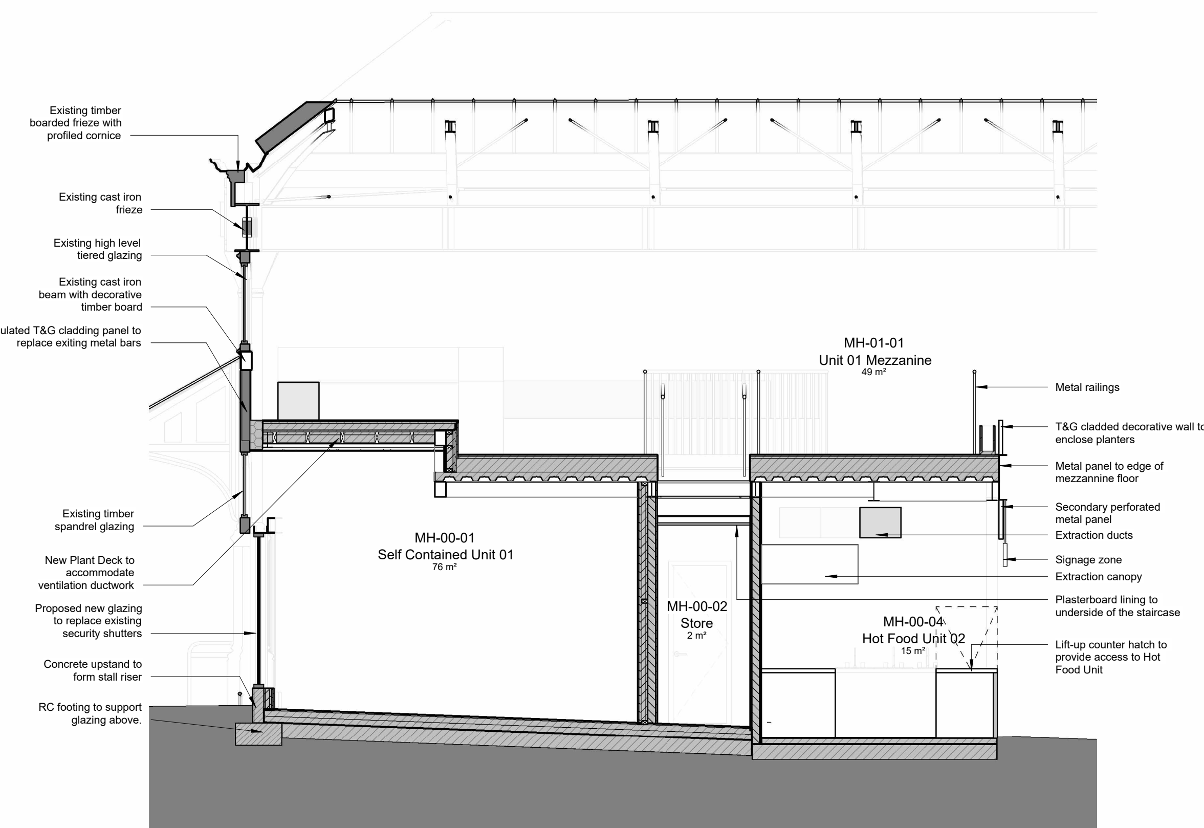
4 Byram St. Self Contained Unit 01 - Section 2 1 : 50
