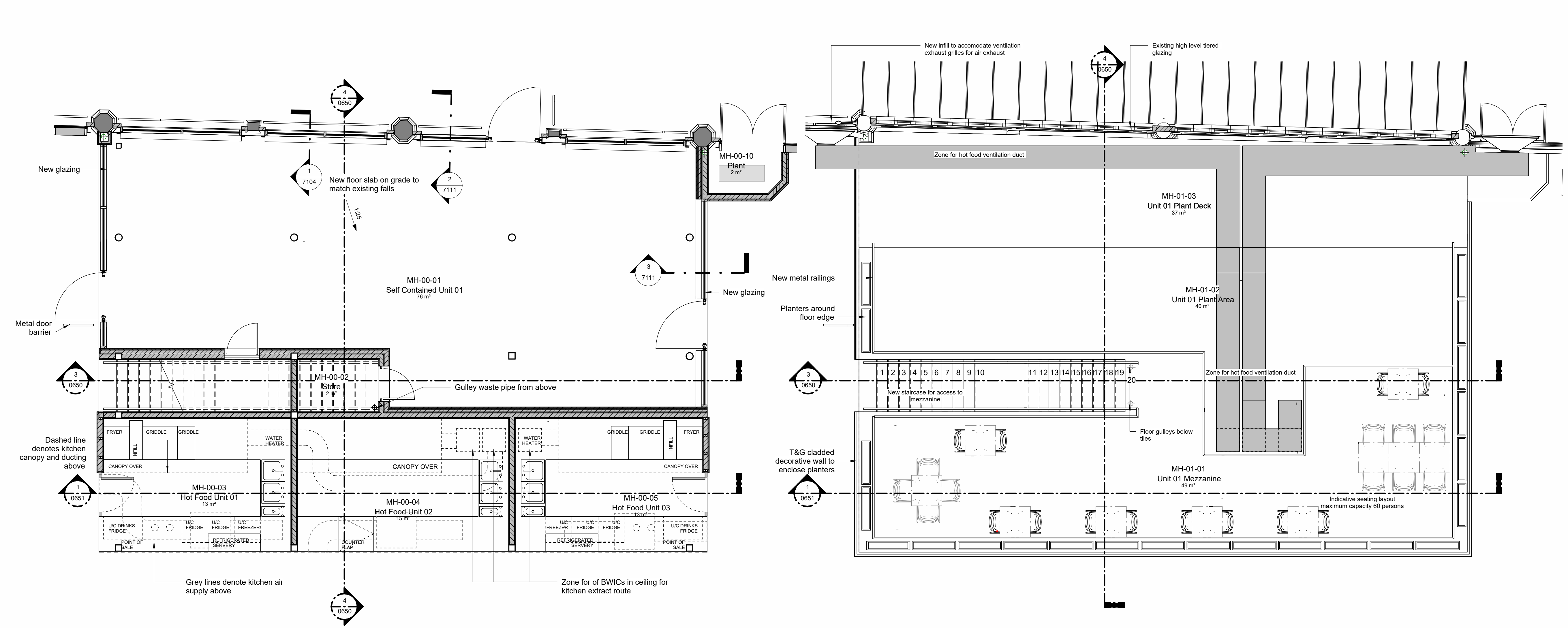
1 Byram St. Self Contained Unit 01 - Level 00 1 : 50
