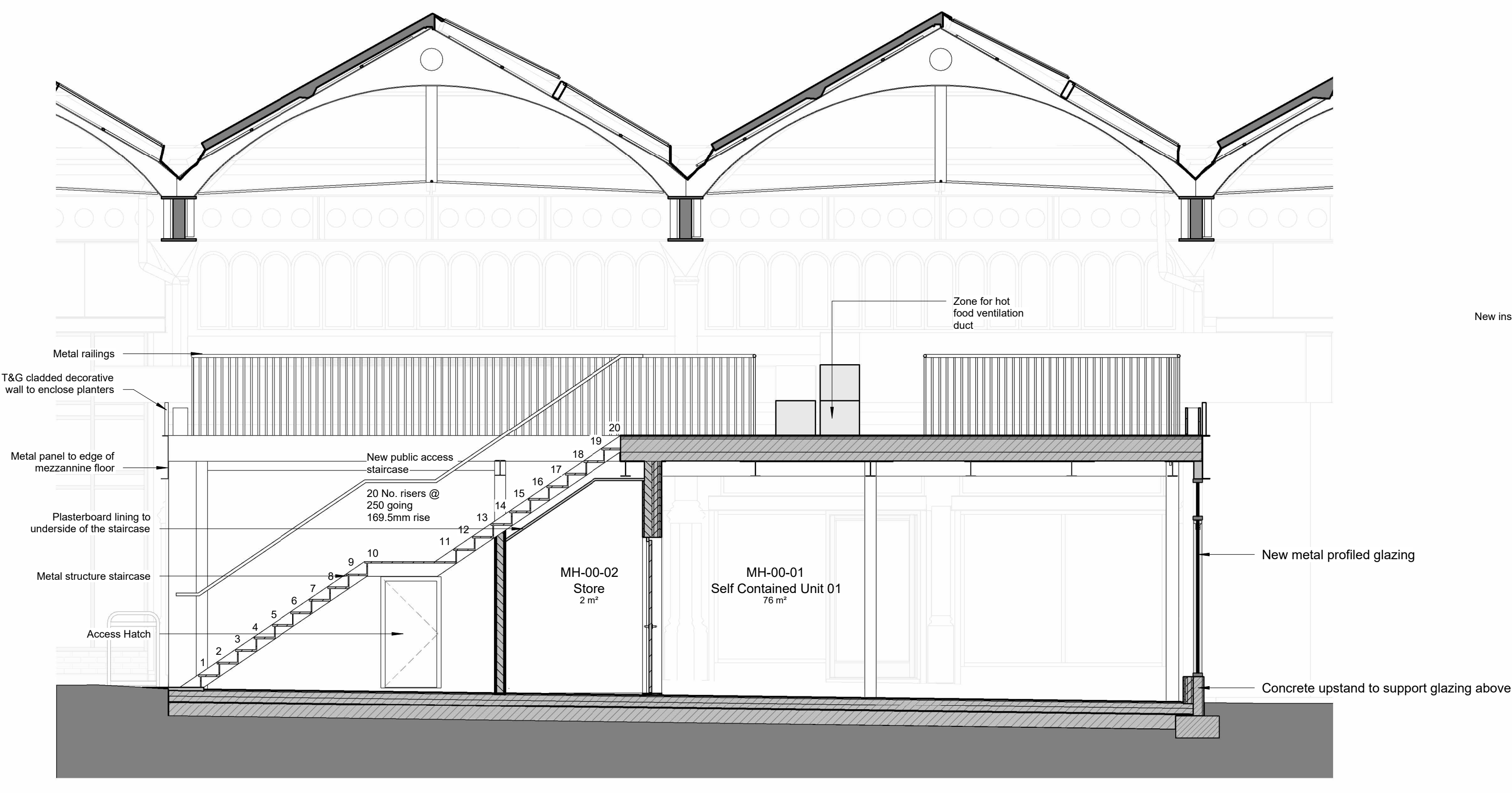
3 Byram St. Self Contained Unit 01 - Section 1 1 : 50
