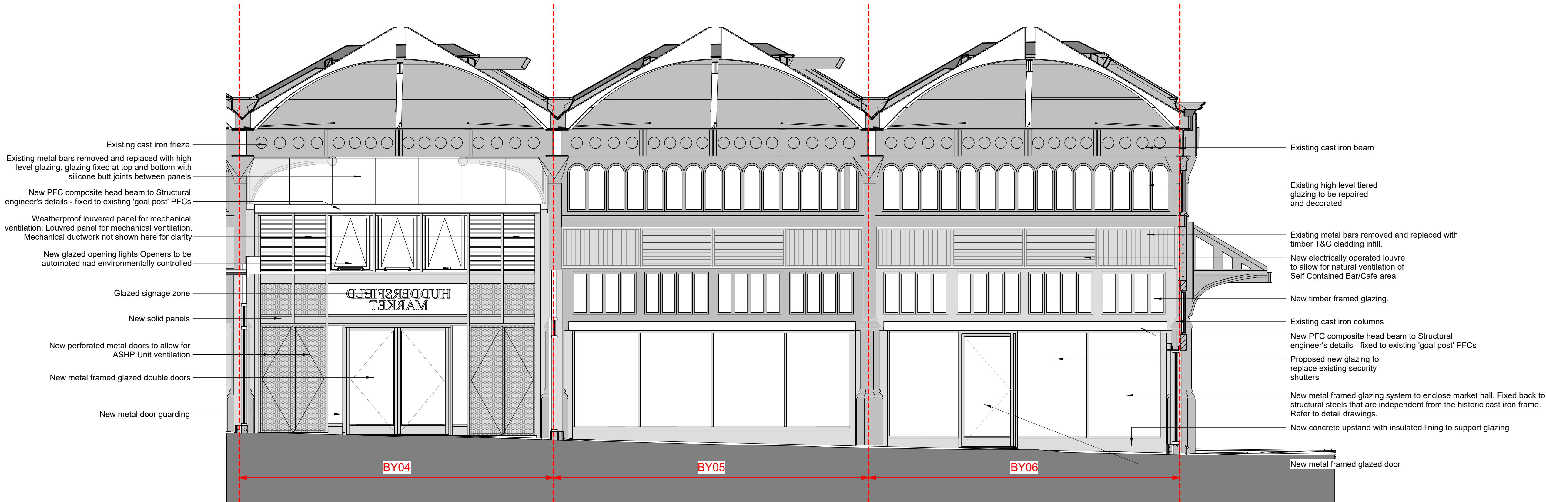
2 BY04-BY06 Internal Elevation 1 : 50
