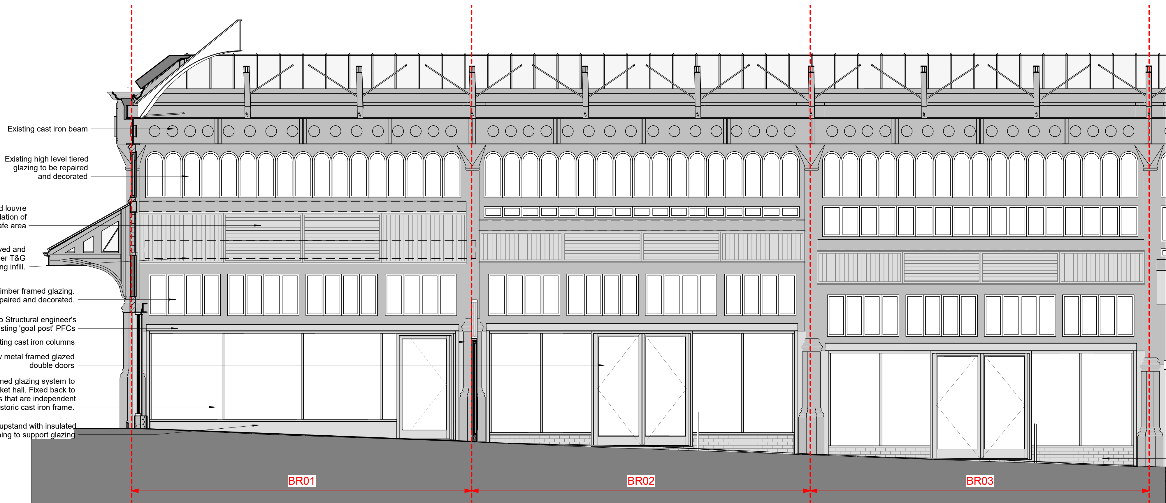
2 BR01-BR03 Internal Elevation 1 : 50
