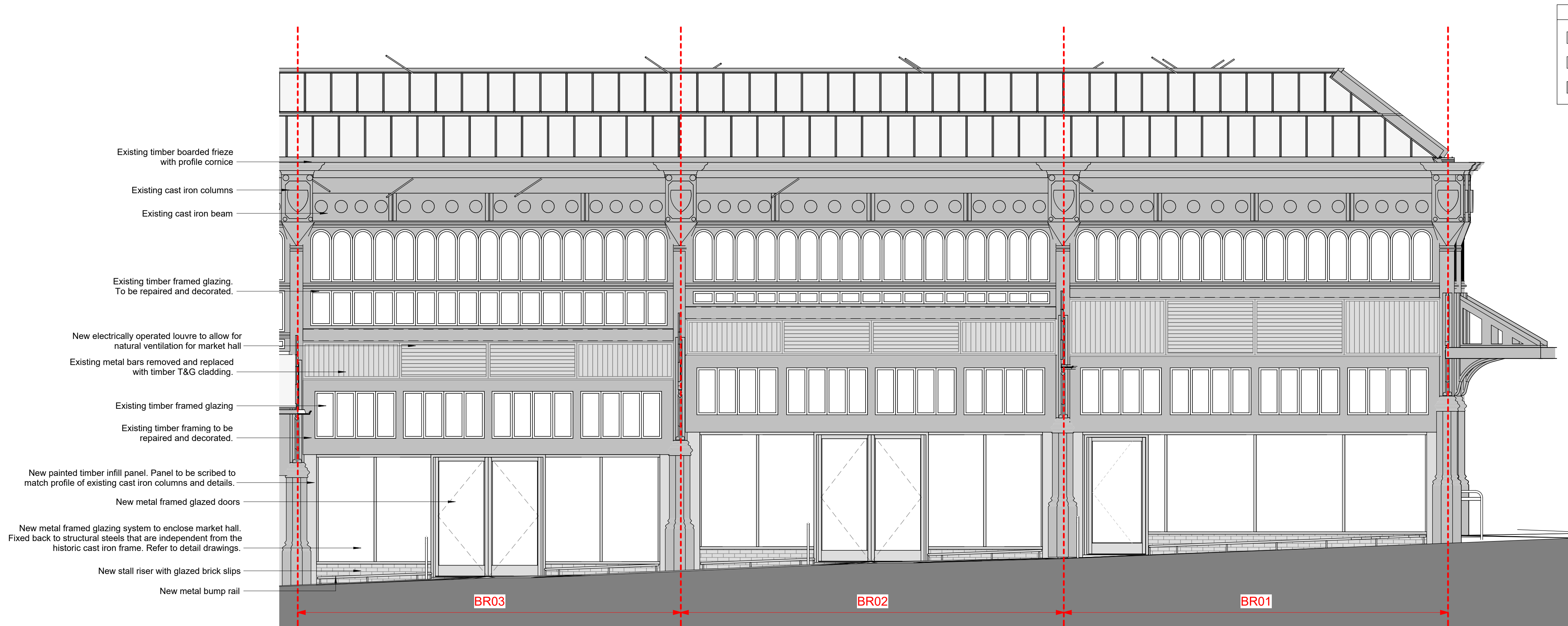
1 BR01-BR03 External Elevation 1 : 50
