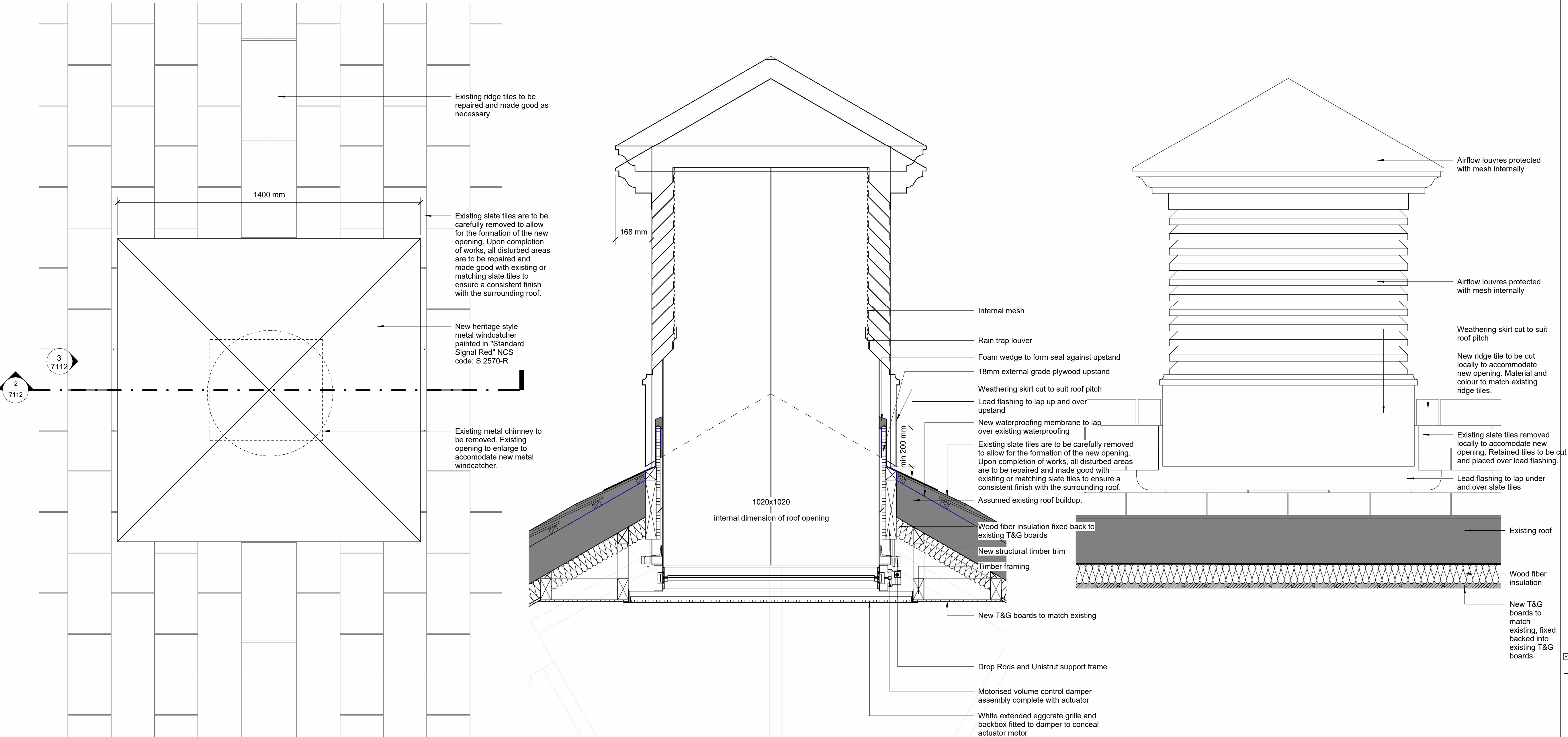
1 Windcatcher Detail - Plan 1 : 10
