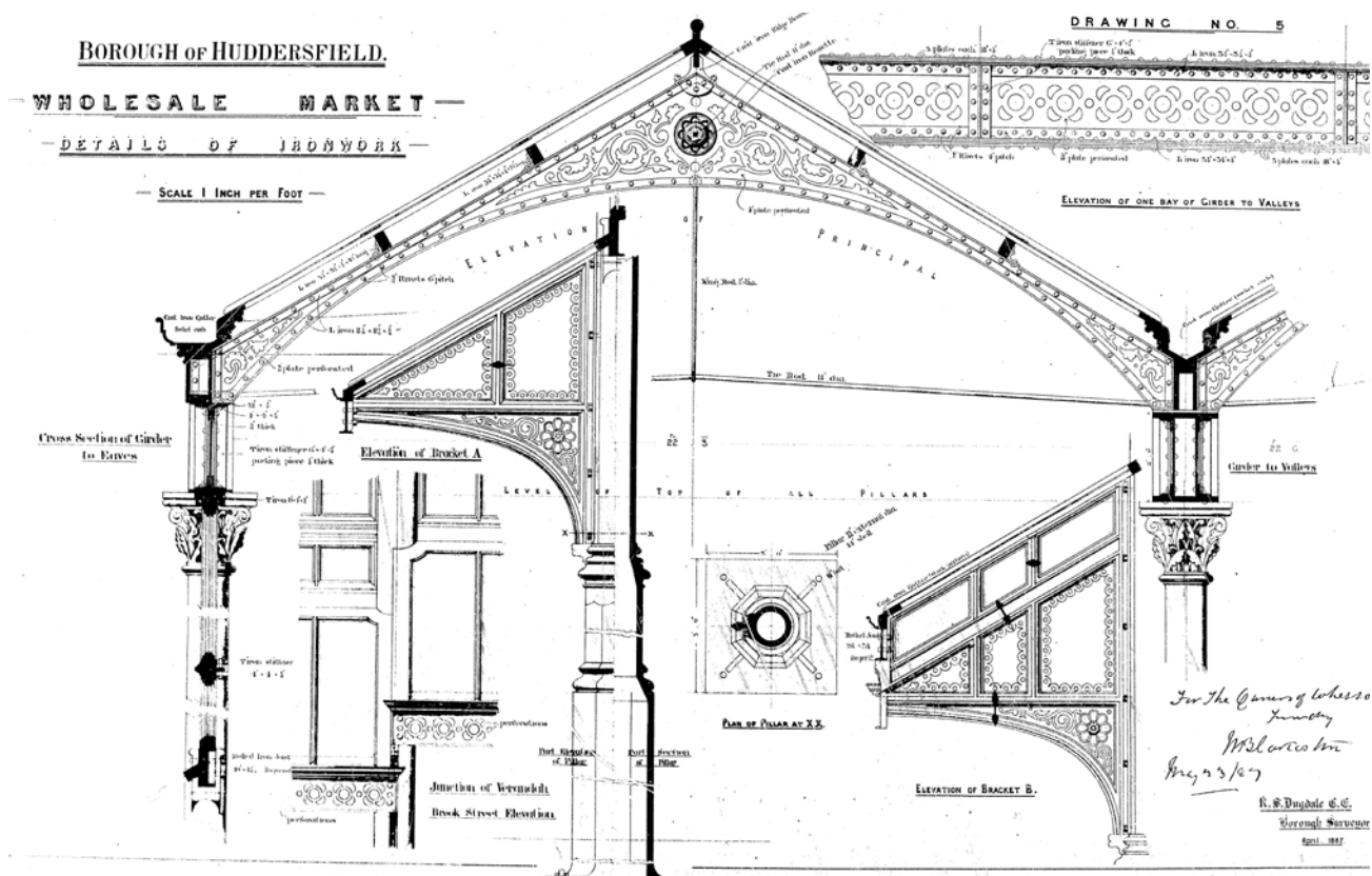
1886 / 87 Ironwork detailing design
