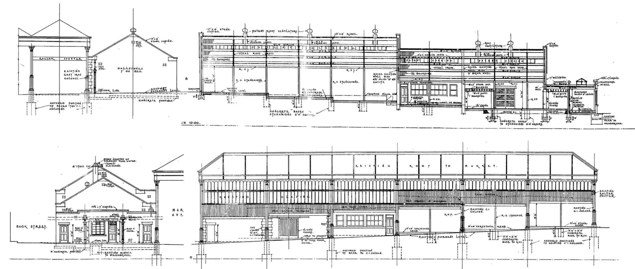
1930's extension drawing showing the design for the Annexe
