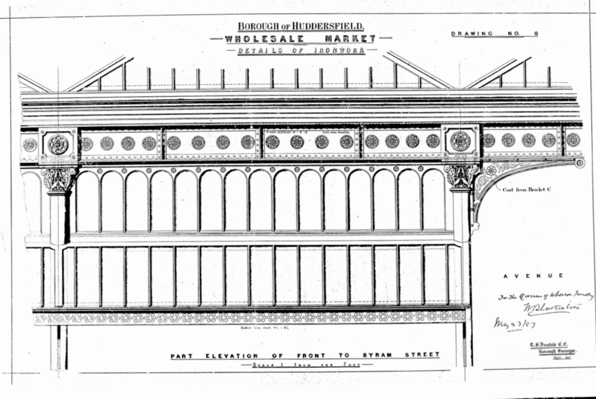
1886 / 87 Ironwork detailing design
