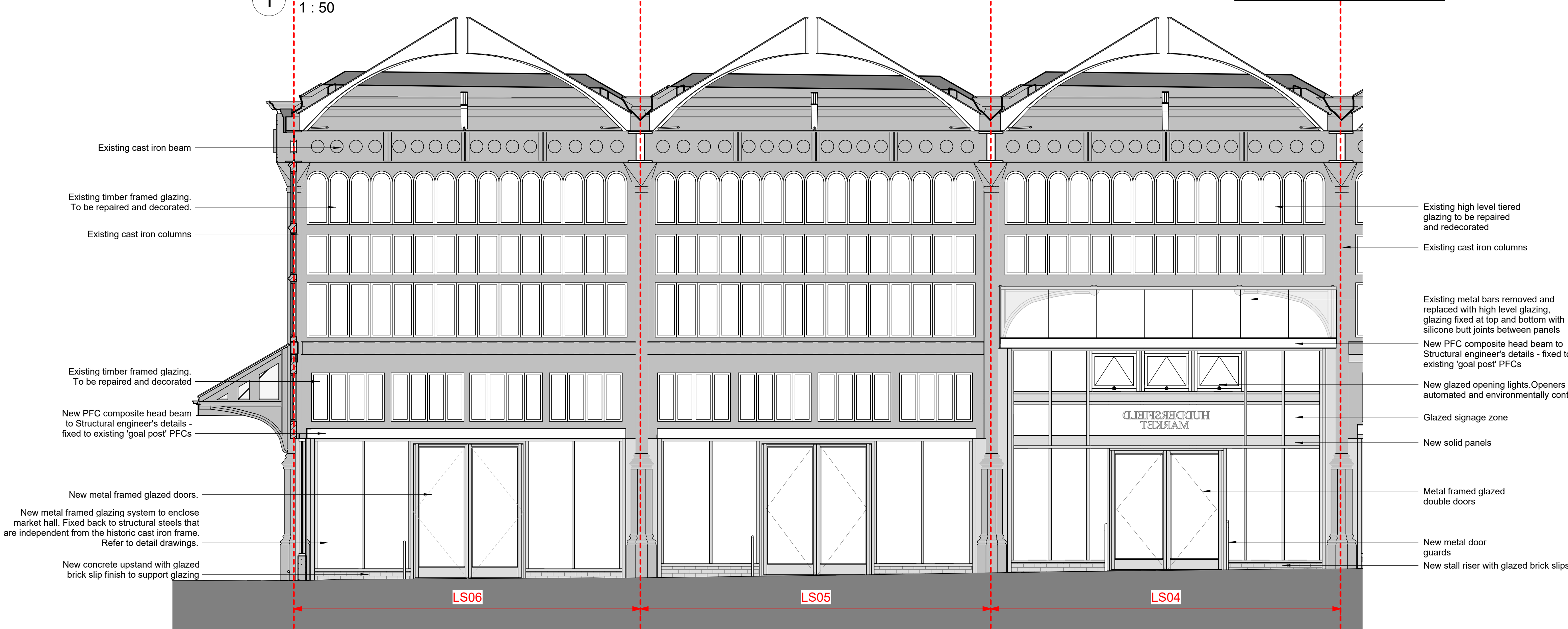
2 LS04-LS06 Internal Elevation 1 : 50
