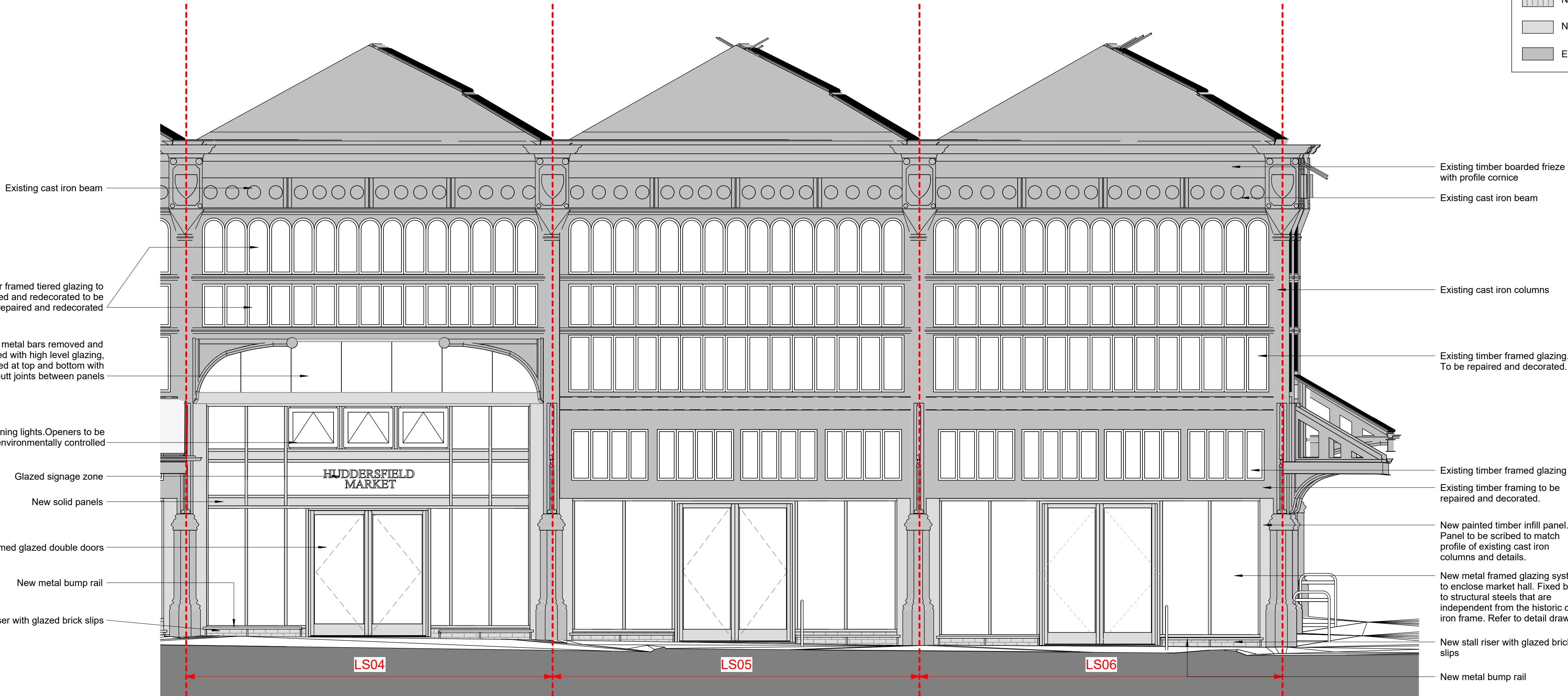
1 LS04-LS06 External Elevation 1 : 50
