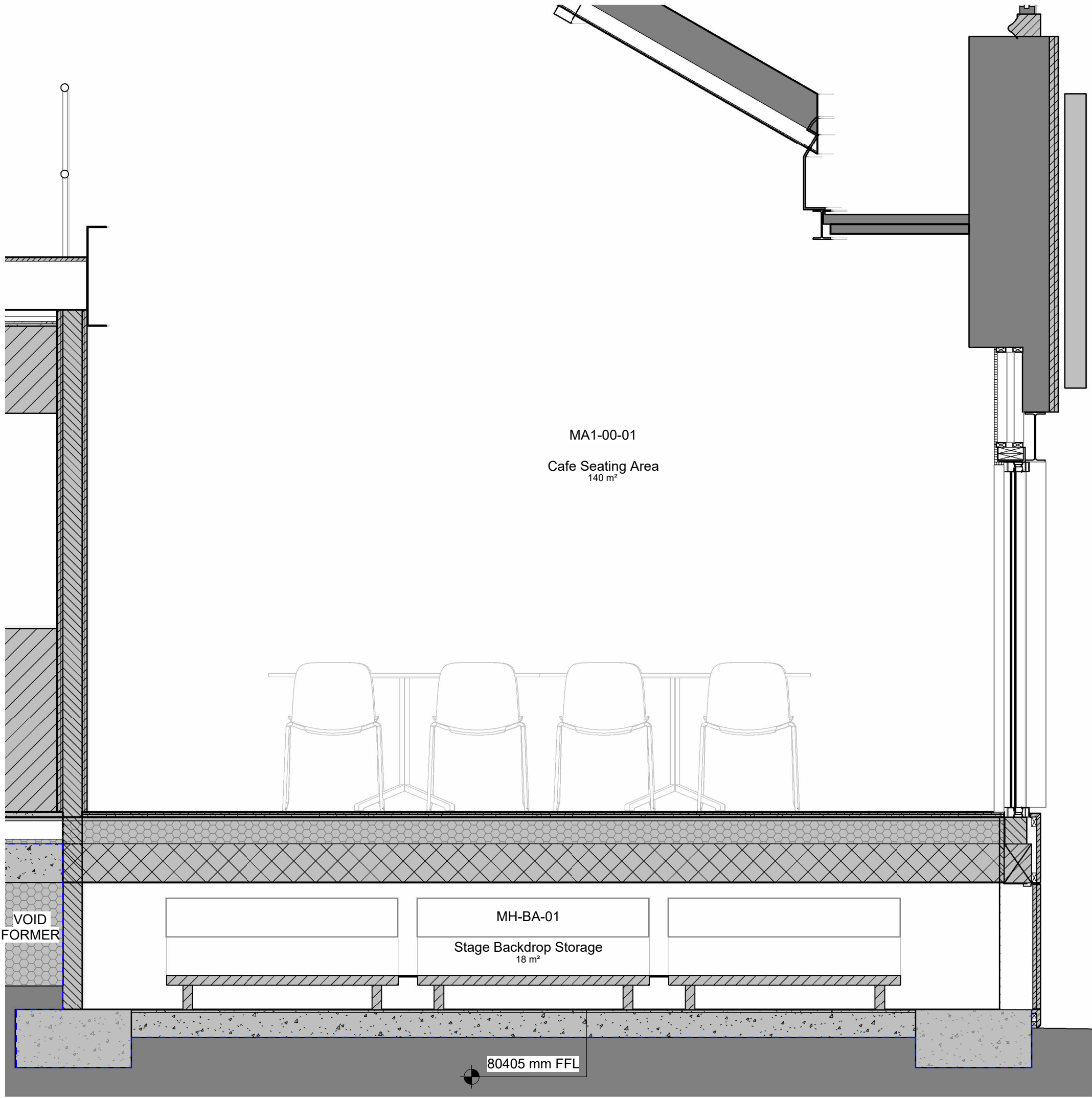
3 Stage Backdrop Storage Section 1 : 20
