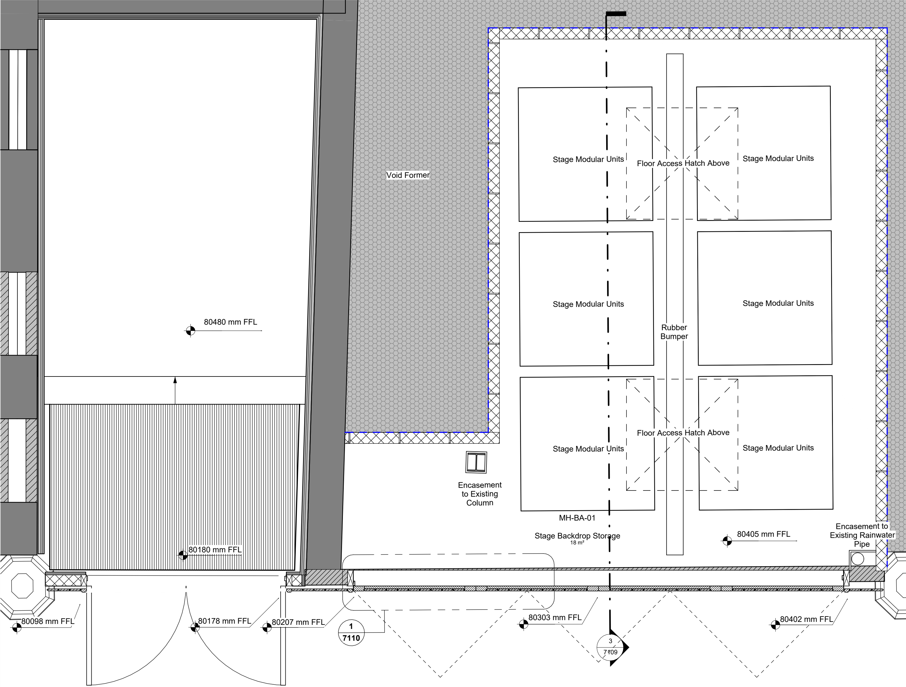
1 Stage Backdrop Storage Plan 1 : 20
