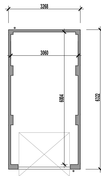
Floor Plan
