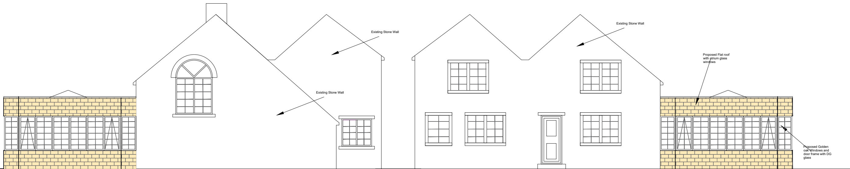
PROPOSED REAR ELEVATION (South West)
