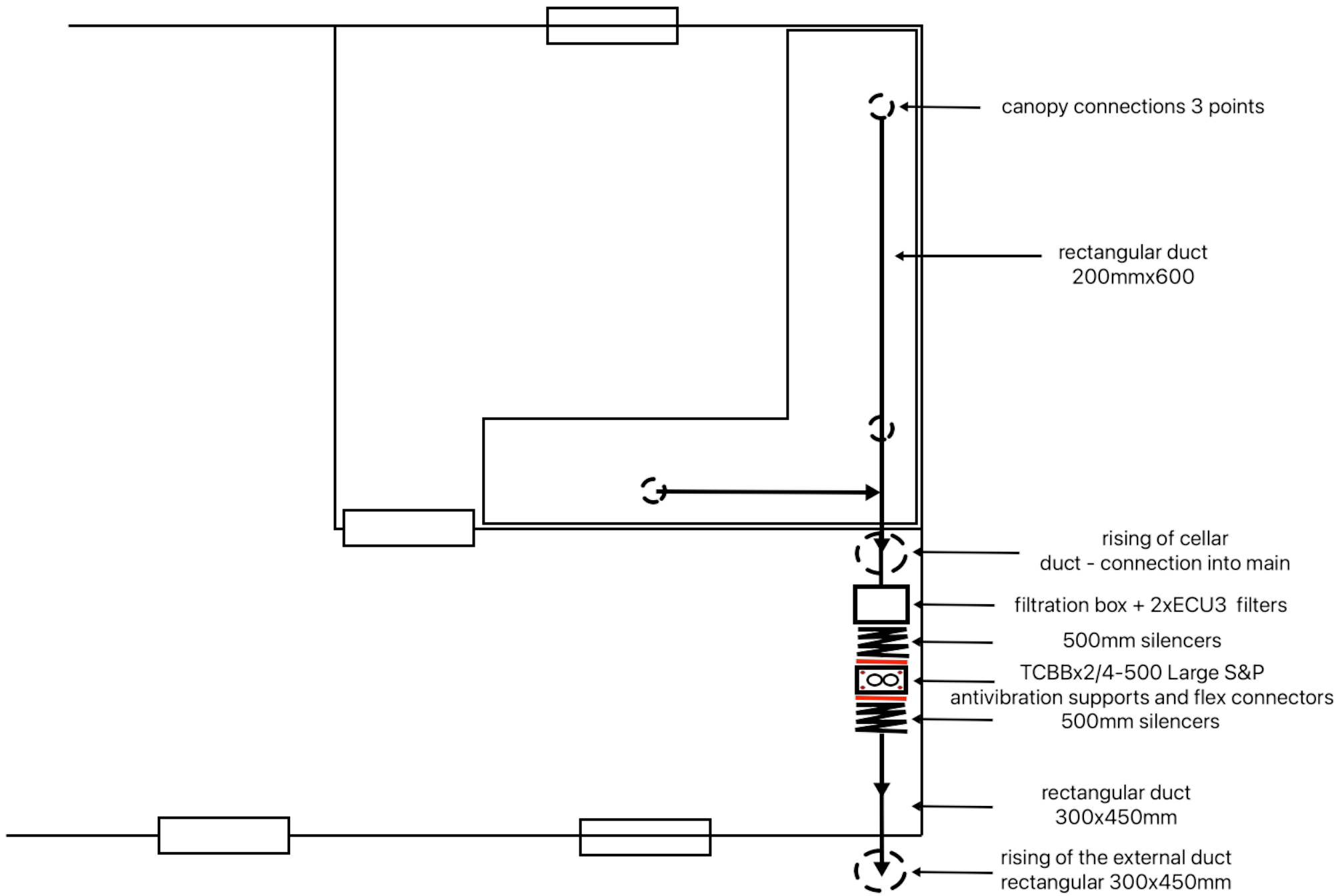
First floor Proposed extract system
