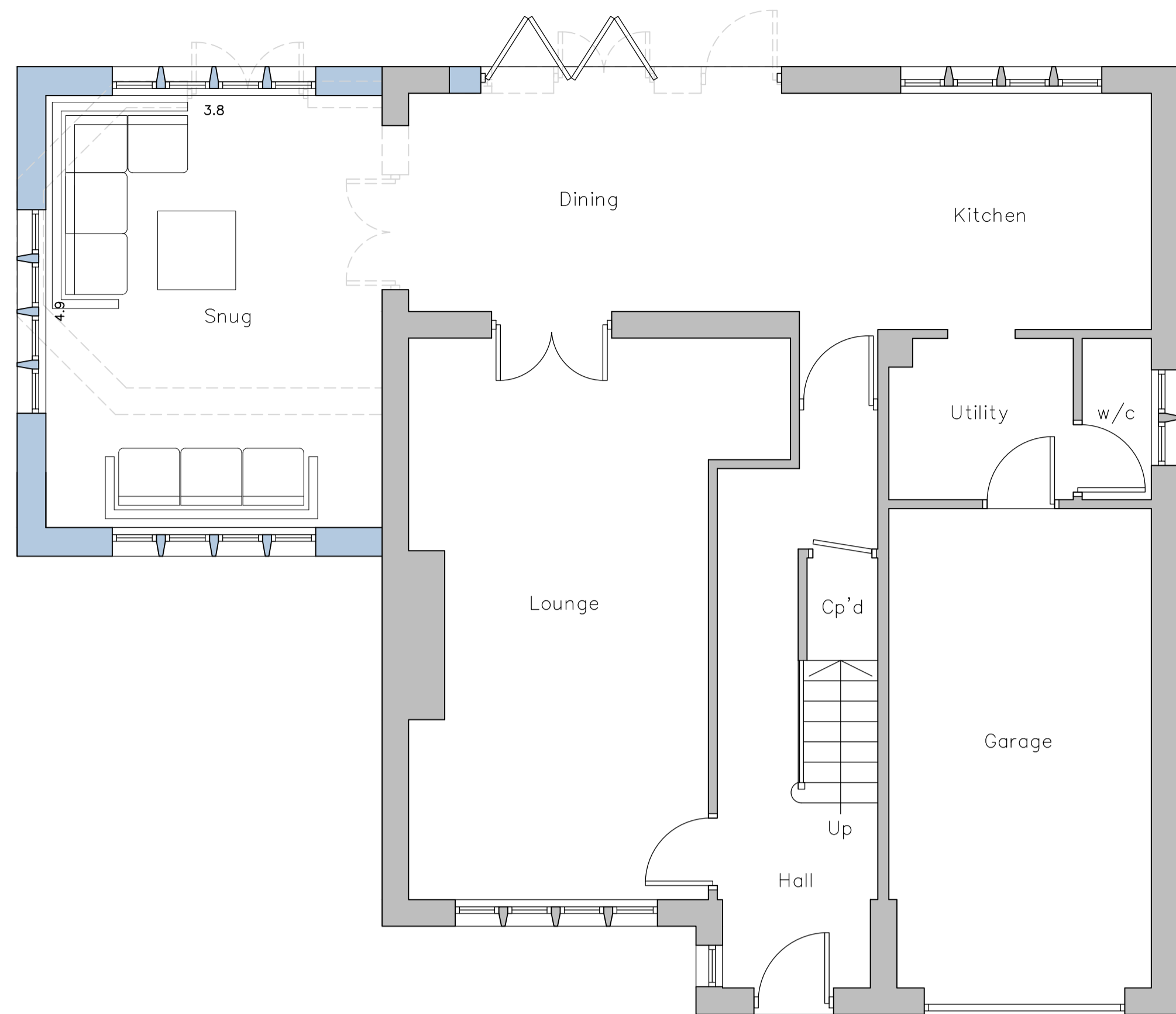
Proposed Ground Floor Layout Scale 1:50
