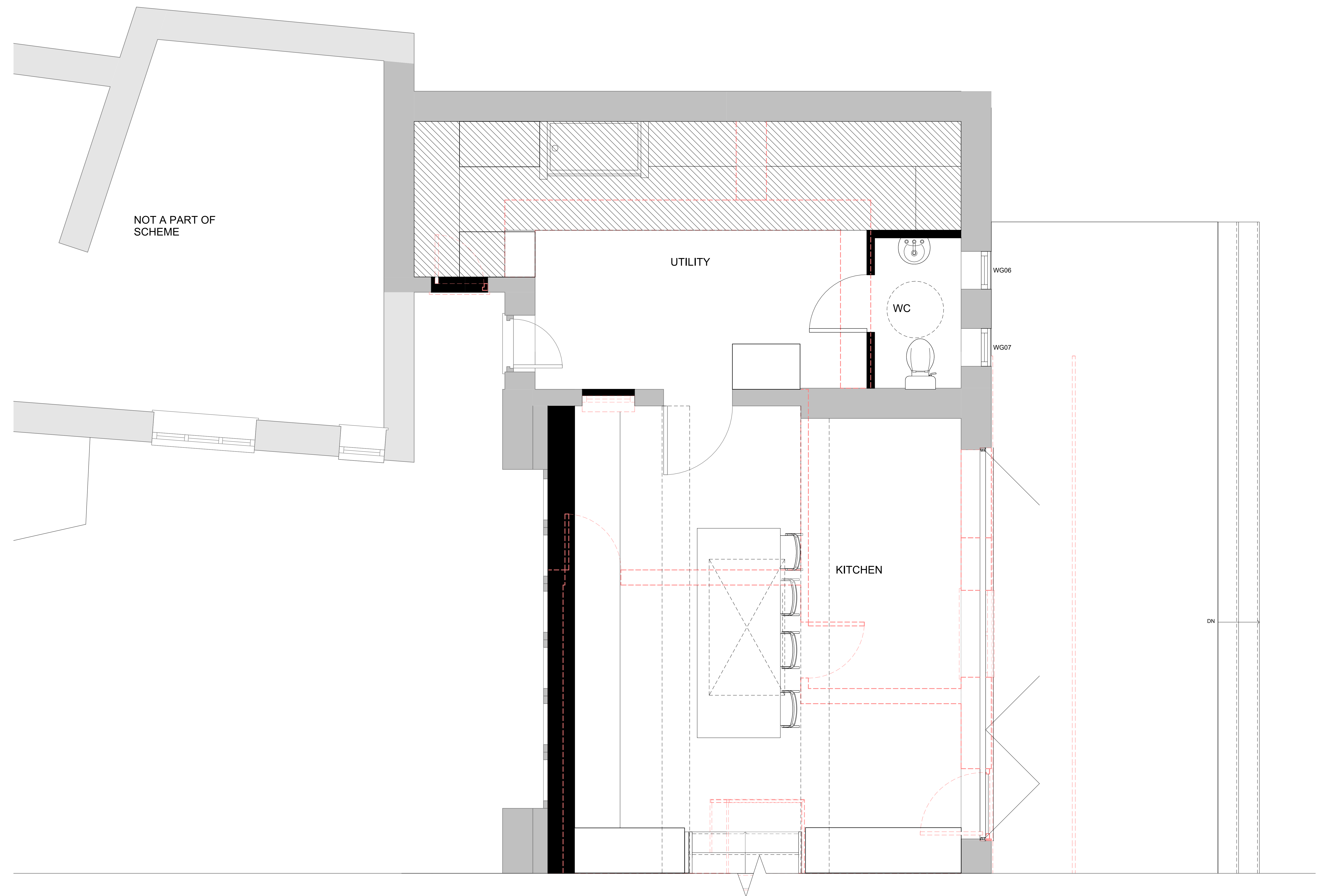
1 Proposed Ground Floor Section Plan 2 1:20
