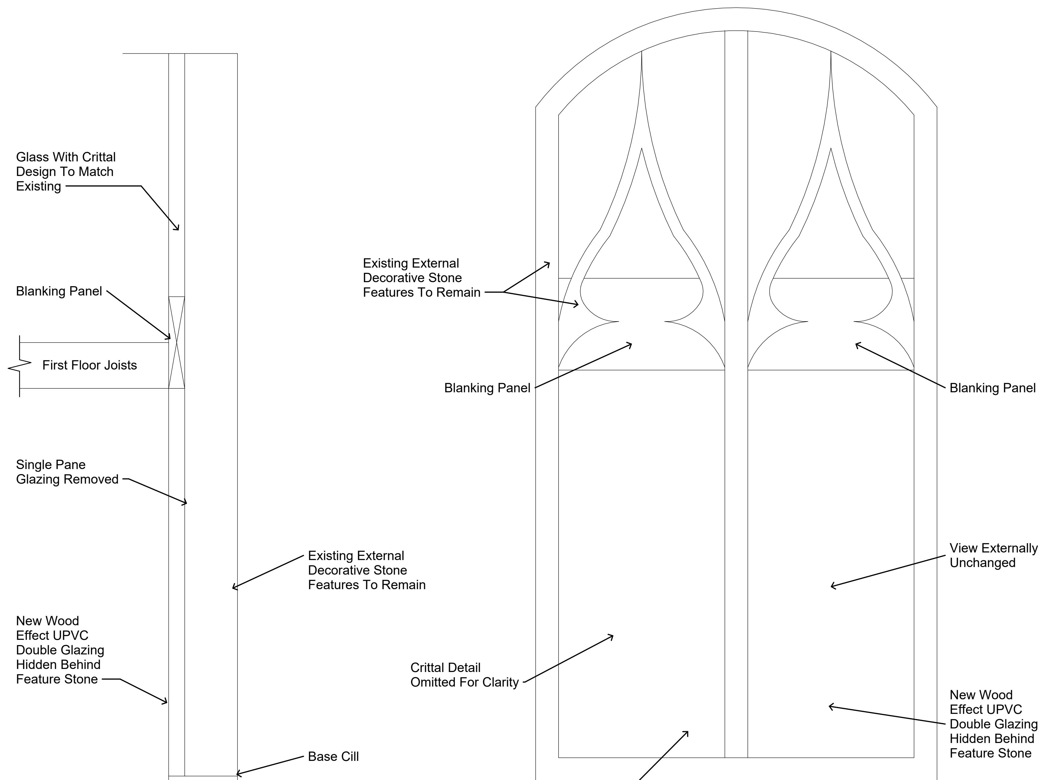
Window Section
