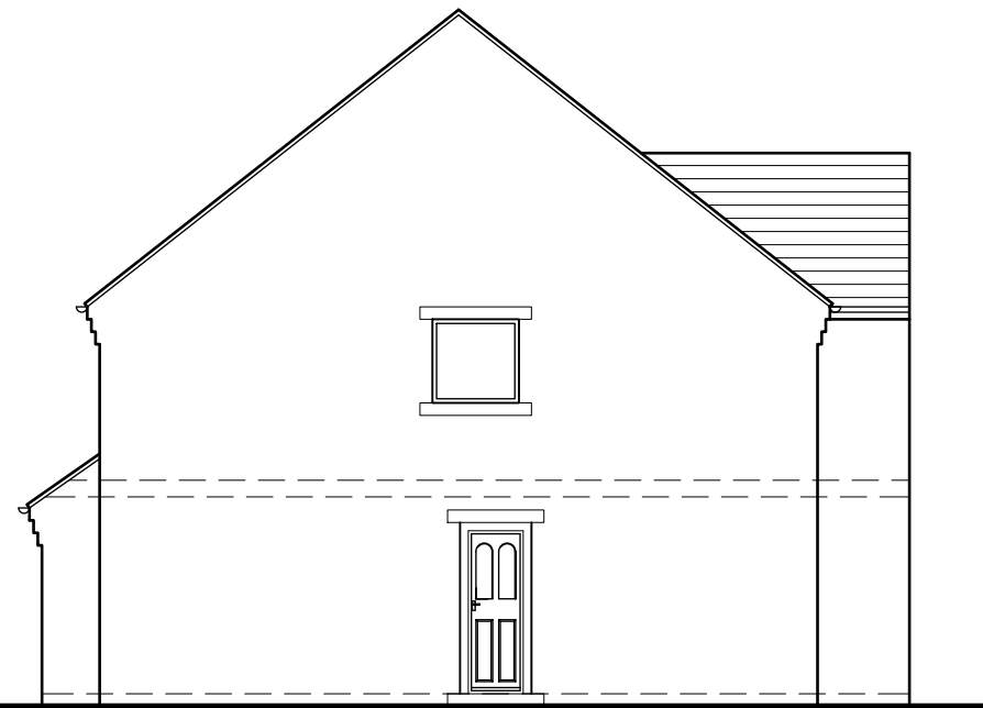
NORTH ELEVATION
