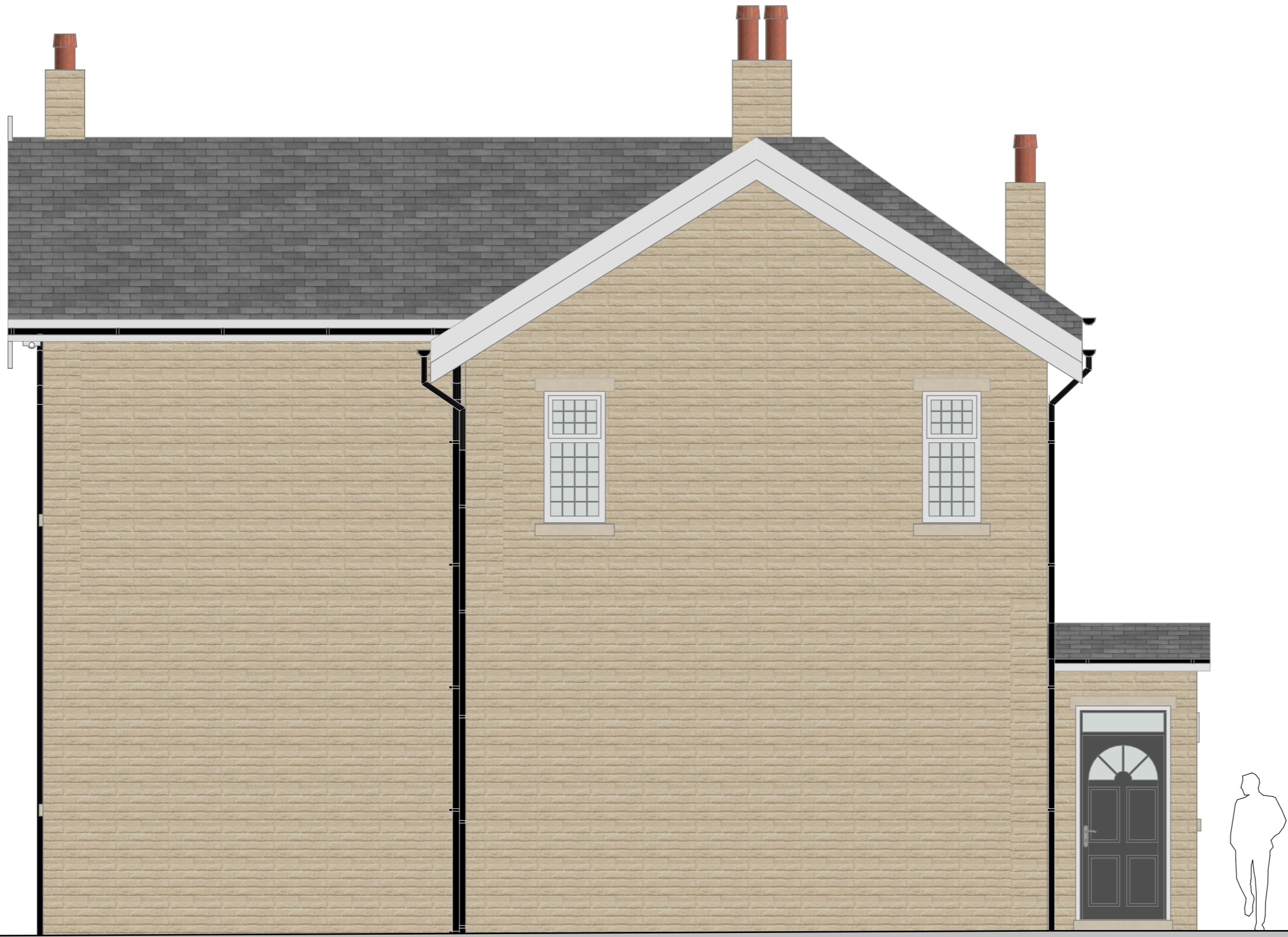
EXISTING REAR ELEVATION 1:50@A3
