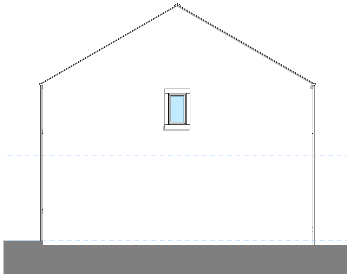
Side Elevation 1:75
