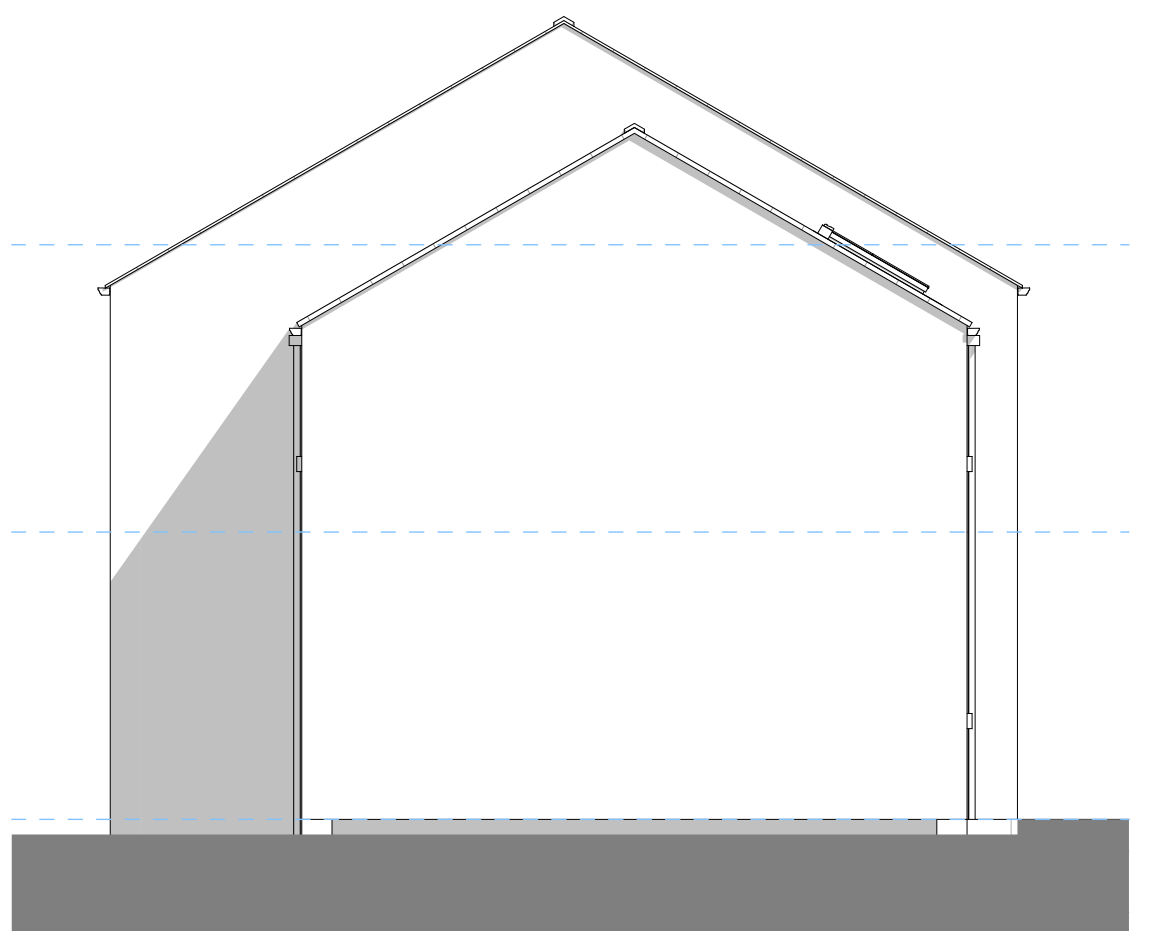
Side Elevation 1:75
