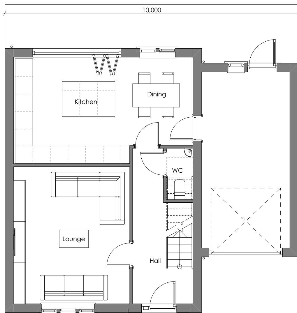
HTF1 Ground Floor 1:75
