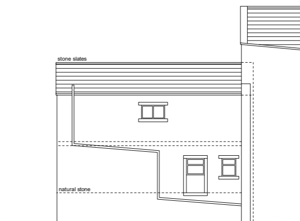
Rear elevation (1:200)
