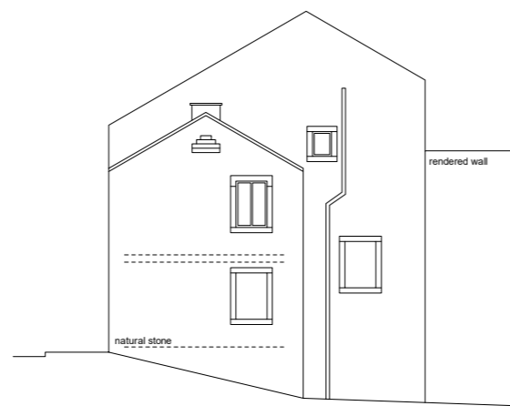
Side elevation (1:200)
