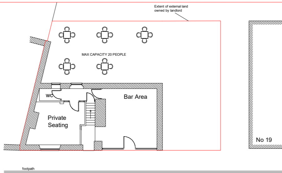
Proposed Ground Floor layout (1:200)
