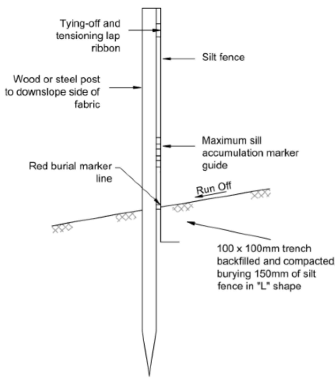
DETAIL 1 - SILT FENCING (NTS)
