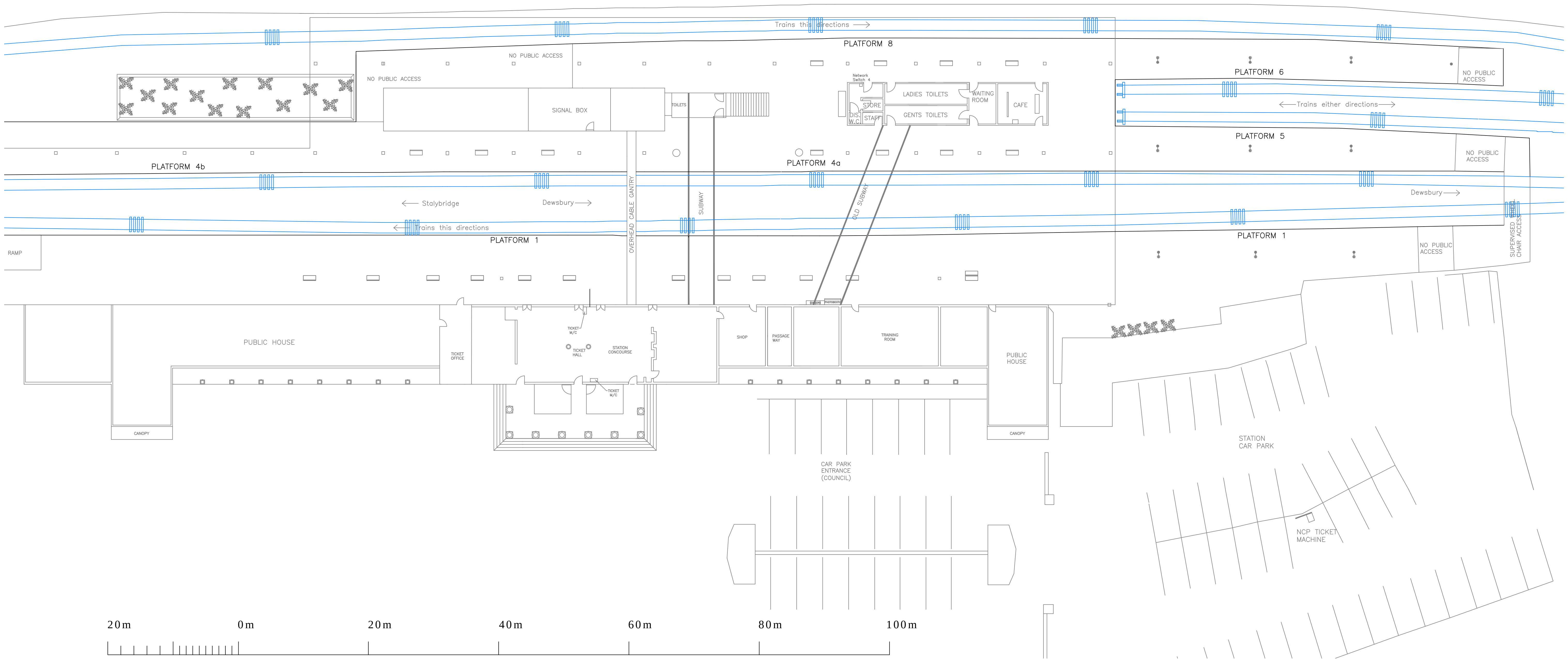
HUDDERSFIELD STATION PLAN - PLATFORM LEVEL SCALE 1:300
