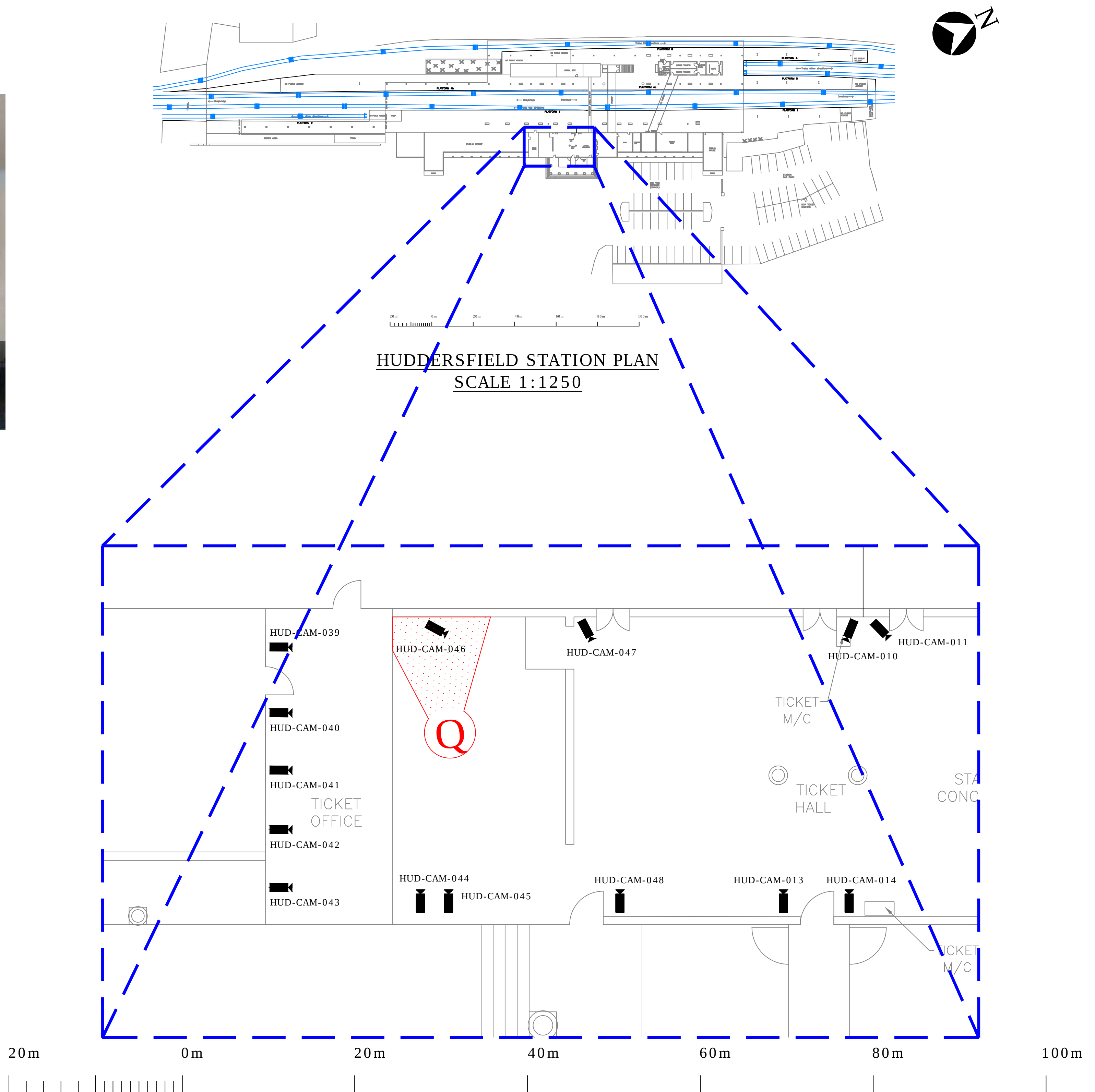
HUDDERSFIELD STATION PLAN - PLATFORM LEVEL SCALE 1:100
