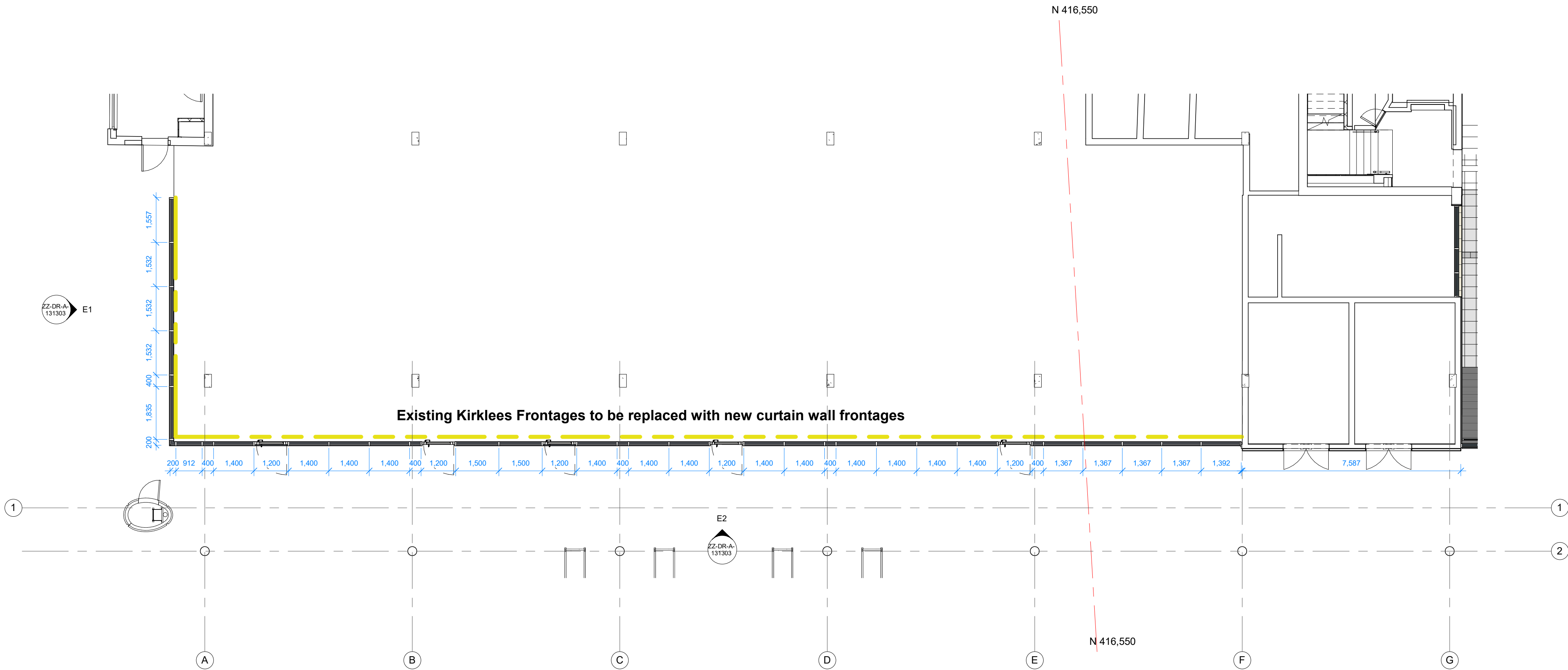
P1 Proposed Kirklees Frontage Plan Scale: 1 : 100
