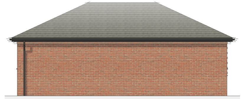
SIDE ELEVATION 2 1 : 100
