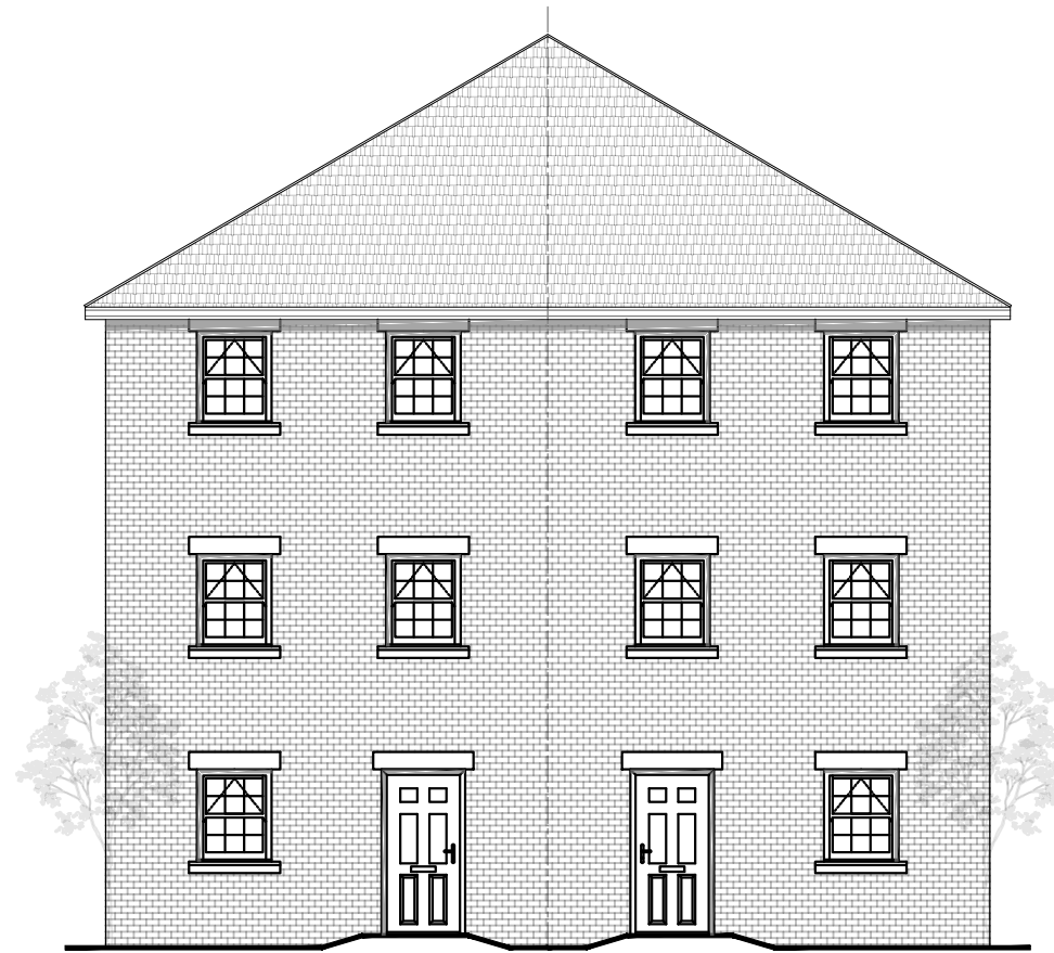
REAR ELEVATION
